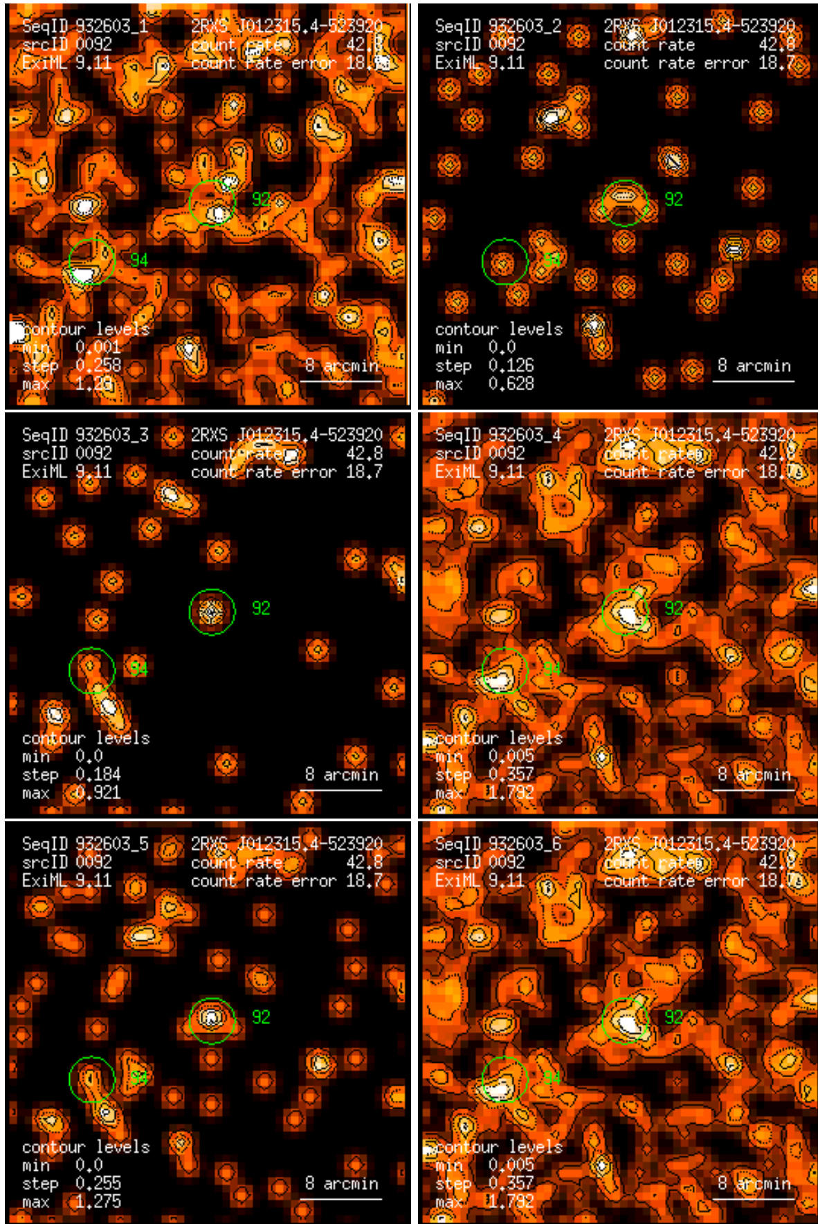
Figure 92: RASS 932603: detection 0092: band rate images, Gaussian filter: (1) PSPP channels 11 – 41, (2) 52 – 90, (3) 91 – 201, (4) 11 – 235, (5) 52 – 201, (6) 11 – 201. Broad band rates in counts/ks. Band rate contour levels in counts/ks/arcmin 2 .
