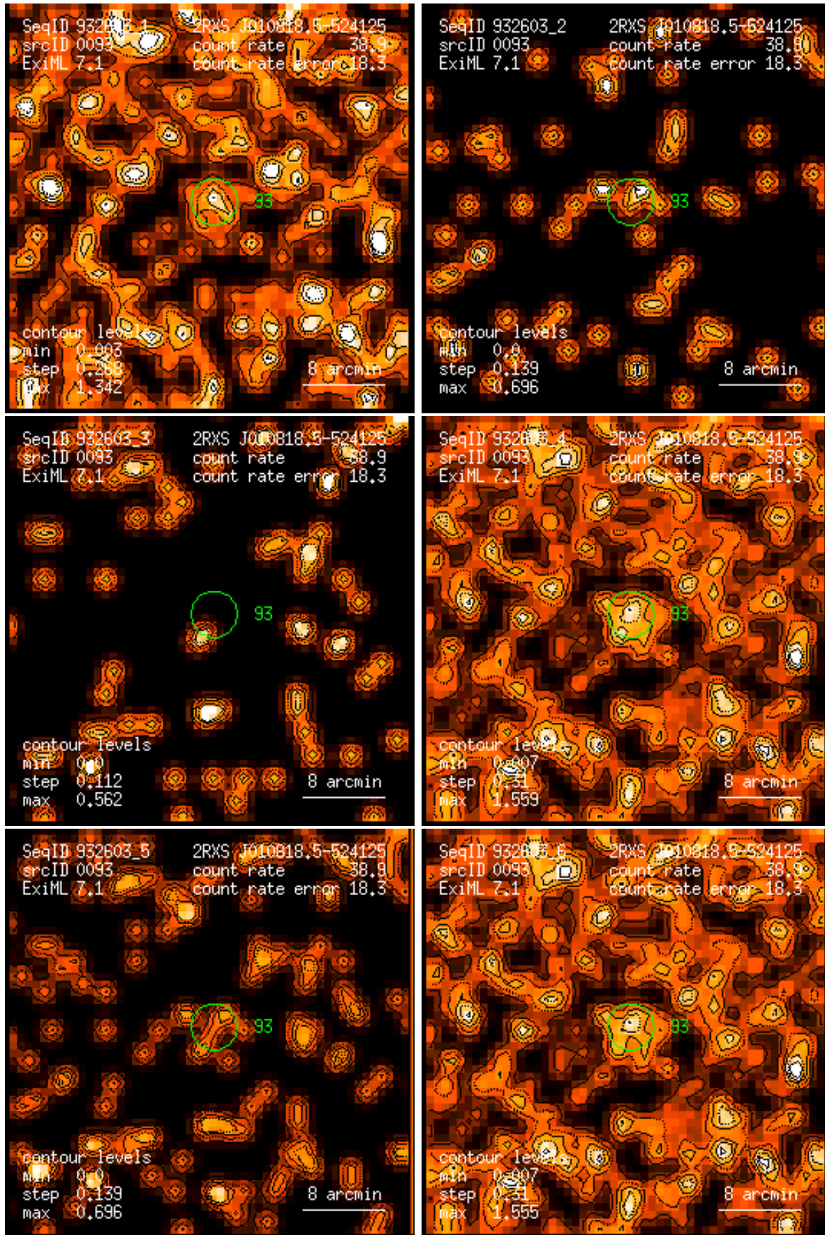
Figure 93: RASS 932603: detection 0093: band rate images, Gaussian filter: (1) PSPC channels 11 – 41, (2) 52 – 90, (3) 91 – 201, (4) 11 – 235, (5) 52 – 201, (6) 11 – 201. Broad band rates in counts/ks. Band rate contour levels in counts/ks/arcmin 2 .
