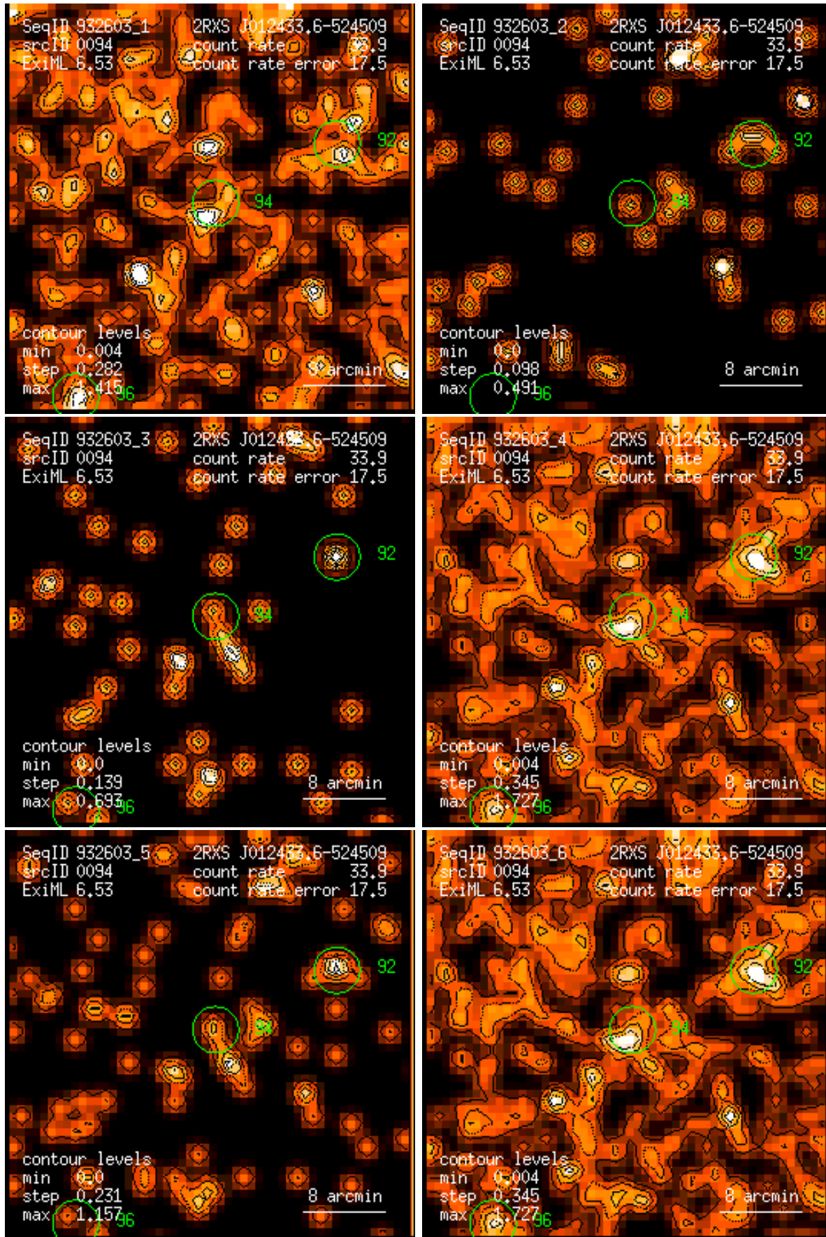
Figure 94: RASS 932603: detection 0094: band rate images, Gaussian filter: (1) PSPC channels 11 – 41, (2) 52 – 90, (3) 91 – 201, (4) 11 – 235, (5) 52 – 201, (6) 11 – 201. Broad band rates in counts/ks. Band rate contour levels in counts/ks/arcmin 2 .
