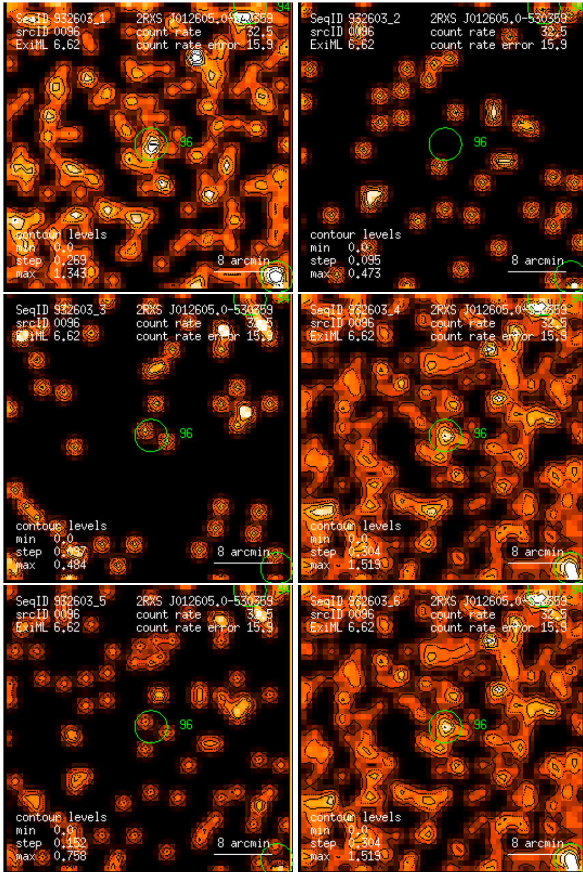
Figure 96: RASS 932603: detection 0096: band rate images, Gaussian filter: (1) PSPC channels 11 – 41, (2) 52 – 90, (3) 91 – 201, (4) 11 – 235, (5) 52 – 201, (6) 11 – 201. Broad band rates in counts/ks. Band rate contour levels in counts/ks/arcmin 2 .
