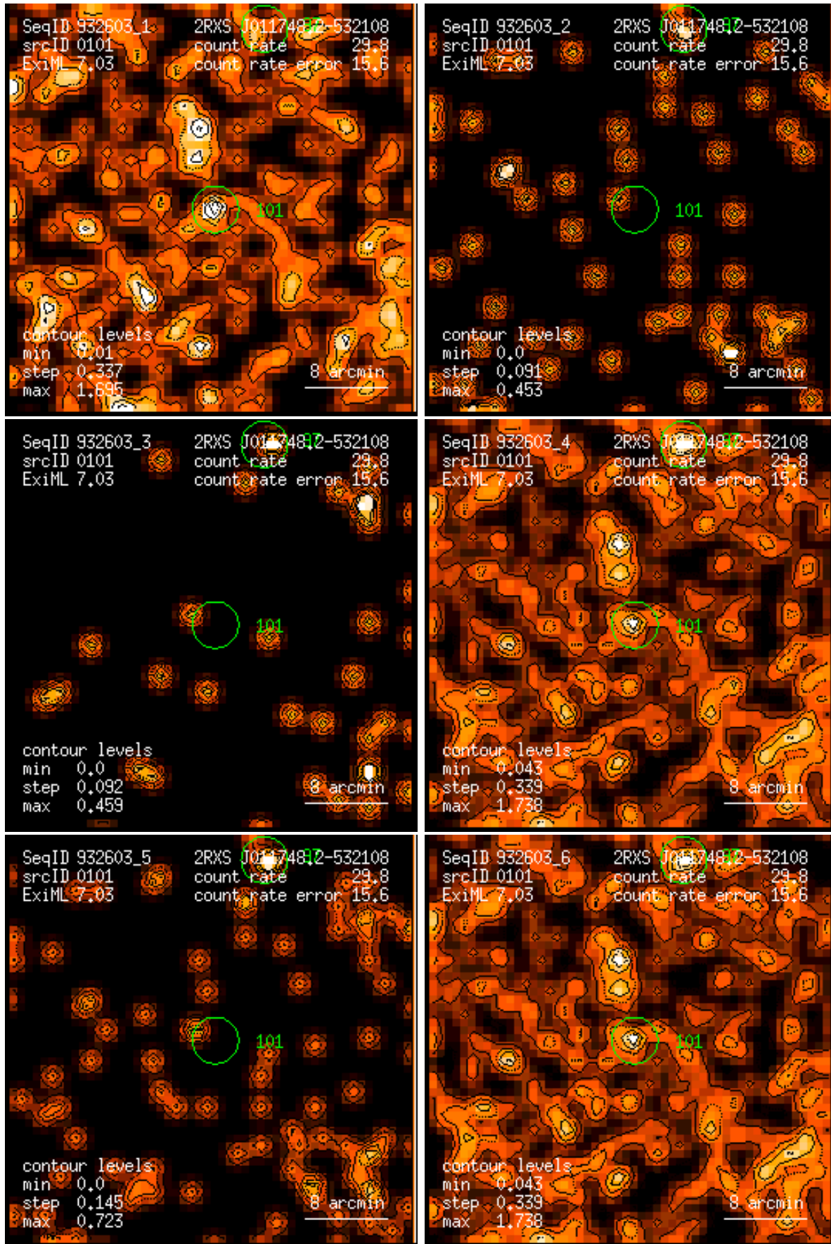
Figure 101: RASS 932603: detection 0101: band rate images, Gaussian filter: (1) PSPC channels 11 – 41, (2) 52 – 90, (3) 91 – 201, (4) 11 – 235, (5) 52 – 201, (6) 11 – 201. Broad band rates in counts/ks. Band rate contour levels in counts/ks/arcmin 2 .
