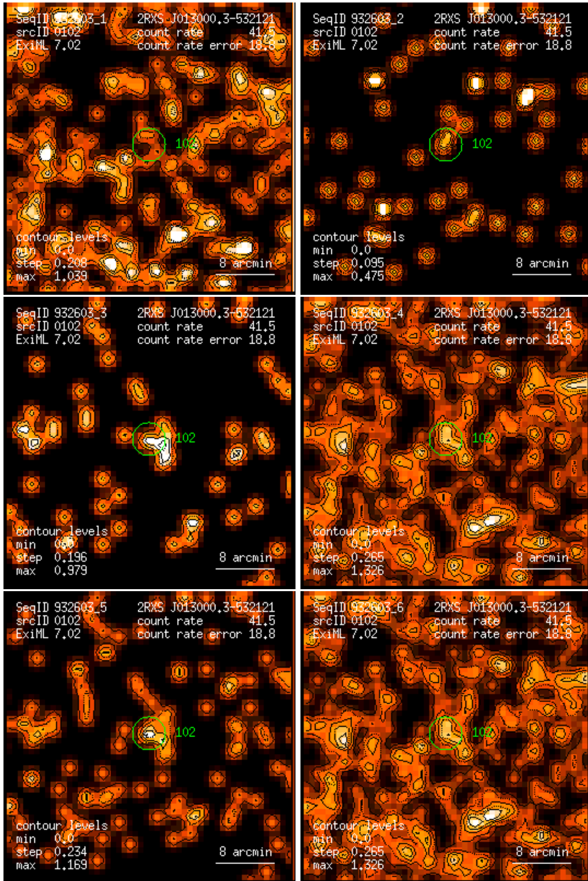
Figure 102: RASS 932603: detection 0102: band rate images, Gaussian filter: (1) PSPC channels 11 – 41, (2) 52 – 90, (3) 91 – 201, (4) 11 – 235, (5) 52 – 201, (6) 11 – 201. Broad band rates in counts/ks. Band rate contour levels in counts/ks/arcmin 2 .
