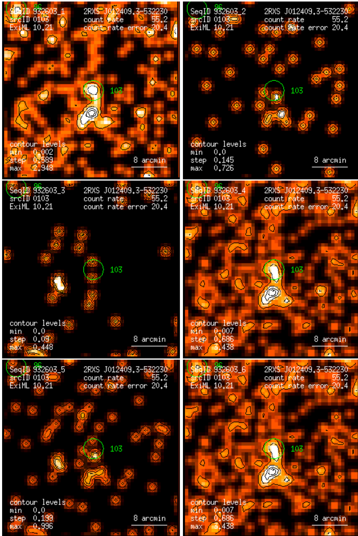
Figure 103: RASS 932603: detection 0103: band rate images, Gaussian filter: (1) PSPC channels 11 – 41, (2) 52 – 90, (3) 91 – 201, (4) 11 – 235, (5) 52 – 201, (6) 11 – 201. Broad band rates in counts/ks. Band rate contour levels in counts/ks/arcmin 2 .
