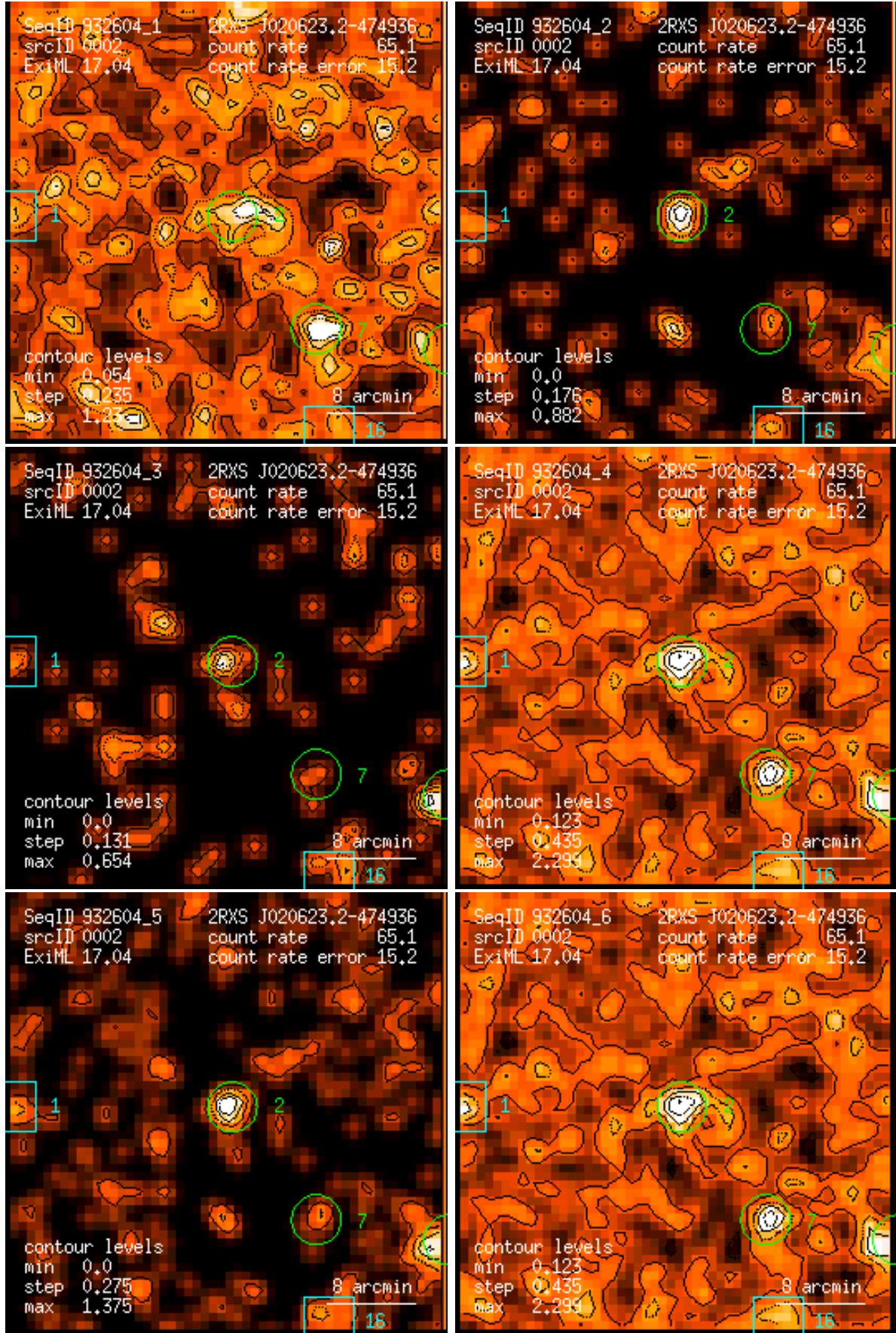
Figure 2: RASS 932604: detection 0002: band rate images, Gaussian filter: (1) PSPC channels 11 – 41, (2) 52 – 90, (3) 91 – 201, (4) 11 – 235, (5) 52 – 201, (6) 11 – 201. Broad band rates in counts/ks. Band rate contour levels in counts/ks/arcmin 2 .
