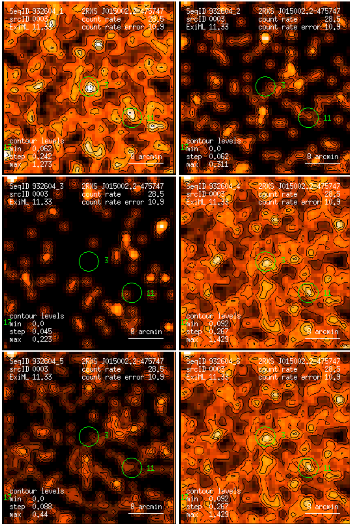
Figure 3: RASS 932604: detection 0003: band rate images, Gaussian filter: (1) PSPC channels 11 – 41, (2) 52 – 90, (3) 91 – 201, (4) 11 – 235, (5) 52 – 201, (6) 11 – 201. Broad band rates in counts/ks. Band rate contour levels in counts/ks/arcmin 2 .
