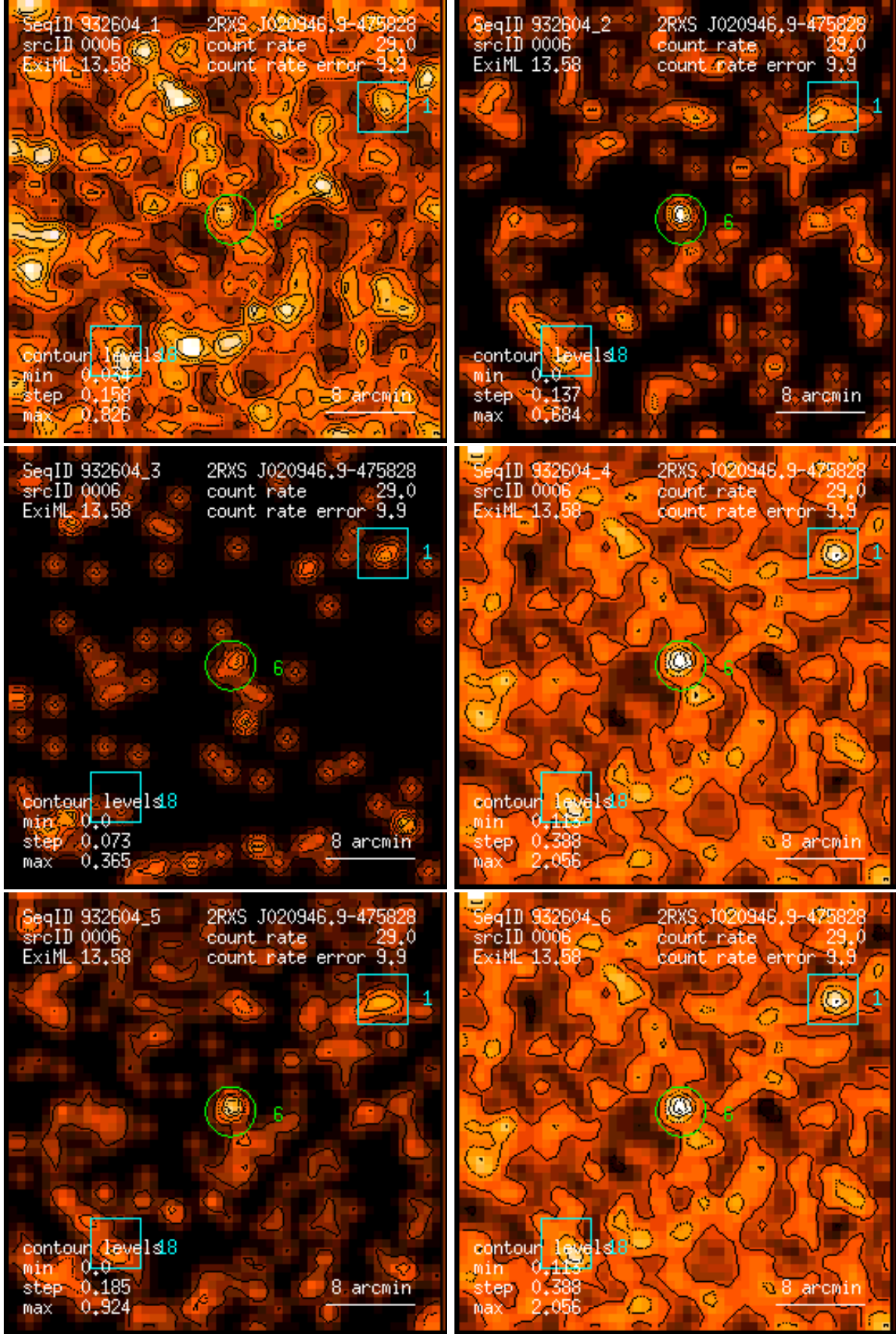
Figure 6: RASS 932604: detection 0006: band rate images, Gaussian filter: (1) PSPC channels 11 – 41, (2) 52 – 90, (3) 91 – 201, (4) 11 – 235, (5) 52 – 201, (6) 11 – 201. Broad band rates in counts/ks. Band rate contour levels in counts/ks/arcmin 2 .
