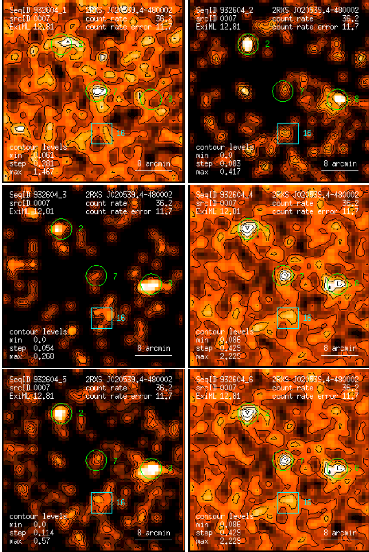
Figure 7: RASS 932604: detection 0007: band rate images, Gaussian filter: (1) PSPC channels 11 – 41, (2) 52 – 90, (3) 91 – 201, (4) 11 – 235, (5) 52 – 201, (6) 11 – 201. Broad band rates in counts/ks. Band rate contour levels in counts/ks/arcmin 2 .
