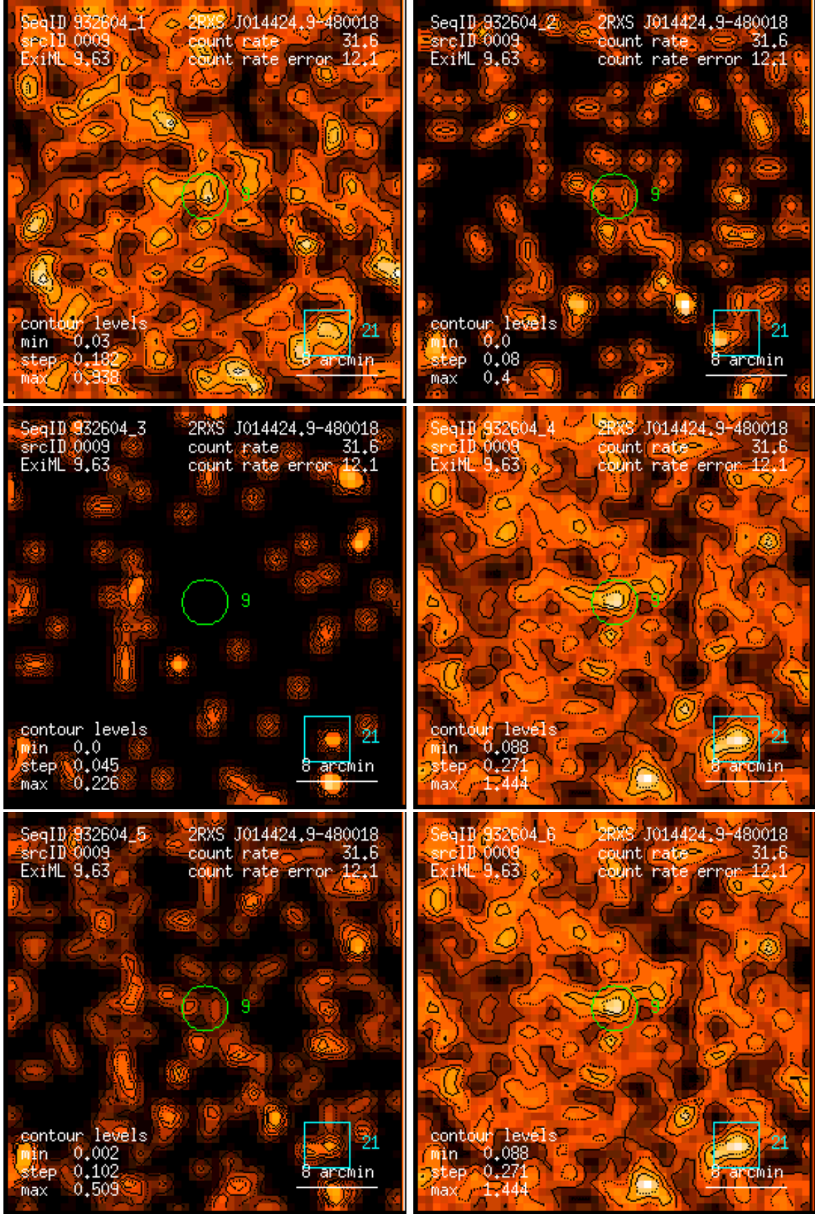
Figure 9: RASS 932604: detection 0009: band rate images, Gaussian filter: (1) PSPC channels 11 – 41, (2) 52 – 90, (3) 91 – 201, (4) 11 – 235, (5) 52 – 201, (6) 11 – 201. Broad band rates in counts/ks. Band rate contour levels in counts/ks/arcmin 2 .
