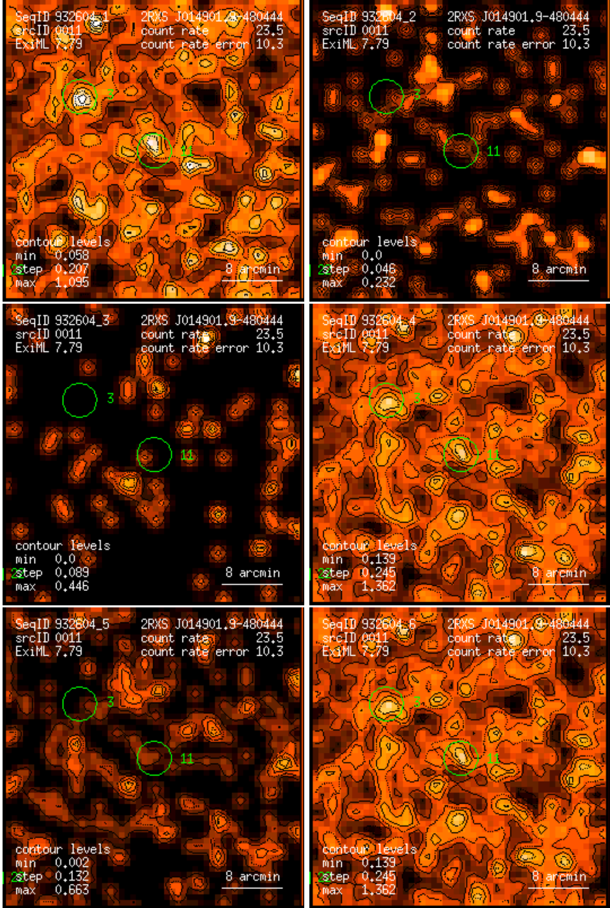
Figure 11: RASS 932604: detection 0011: band rate images, Gaussian filter: (1) PSPC channels 11 – 41, (2) 52 – 90, (3) 91 – 201, (4) 11 – 235, (5) 52 – 201, (6) 11 – 201. Broad band rates in counts/ks. Band rate contour levels in counts/ks/arcmin 2 .
