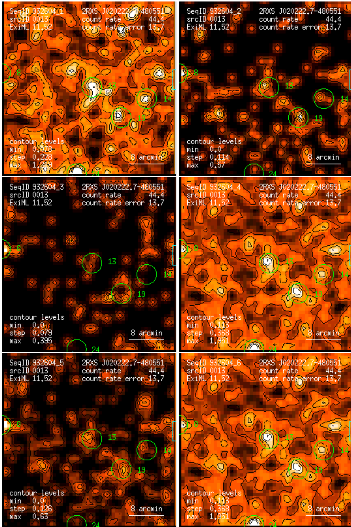
Figure 13: RASS 932604: detection 0013: band rate images, Gaussian filter: (1) PSPC channels 11 – 41, (2) 52 – 90, (3) 91 – 201, (4) 11 – 235, (5) 52 – 201, (6) 11 – 201. Broad band rates in counts/ks. Band rate contour levels in counts/ks/arcmin 2 .
