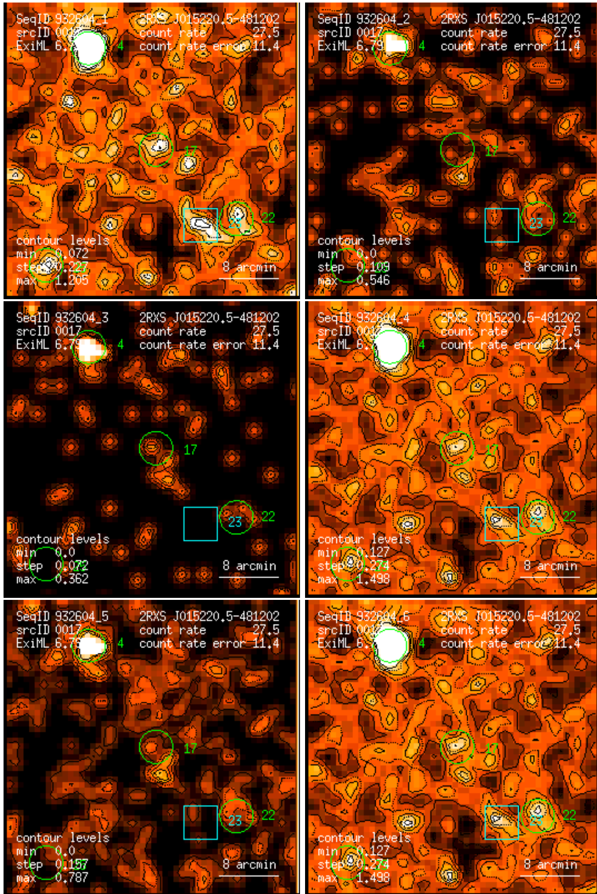
Figure 17: RASS 932604: detection 0017: band rate images, Gaussian filter: (1) PSPC channels 11 – 41, (2) 52 – 90, (3) 91 – 201, (4) 11 – 235, (5) 52 – 201, (6) 11 – 201. Broad band rates in counts/ks. Band rate contour levels in counts/ks/arcmin 2 .
