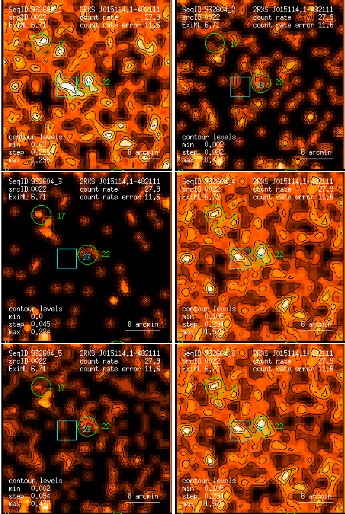
Figure 22: RASS 932604: detection 0022: band rate images, Gaussian filter: (1) PSPC channels 11 – 41, (2) 52 – 90, (3) 91 – 201, (4) 11 – 235, (5) 52 – 201, (6) 11 – 201. Broad band rates in counts/ks. Band rate contour levels in counts/ks/arcmin 2 .
