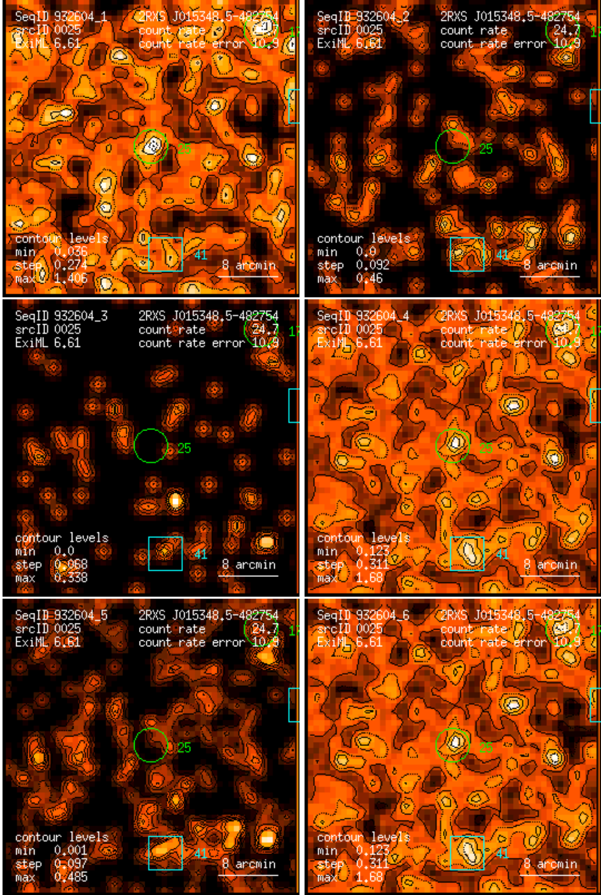
Figure 25: RASS 932604: detection 0025: band rate images, Gaussian filter: (1) PSPC channels 11 – 41, (2) 52 – 90, (3) 91 – 201, (4) 11 – 235, (5) 52 – 201, (6) 11 – 201. Broad band rates in counts/ks. Band rate contour levels in counts/ks/arcmin 2 .
