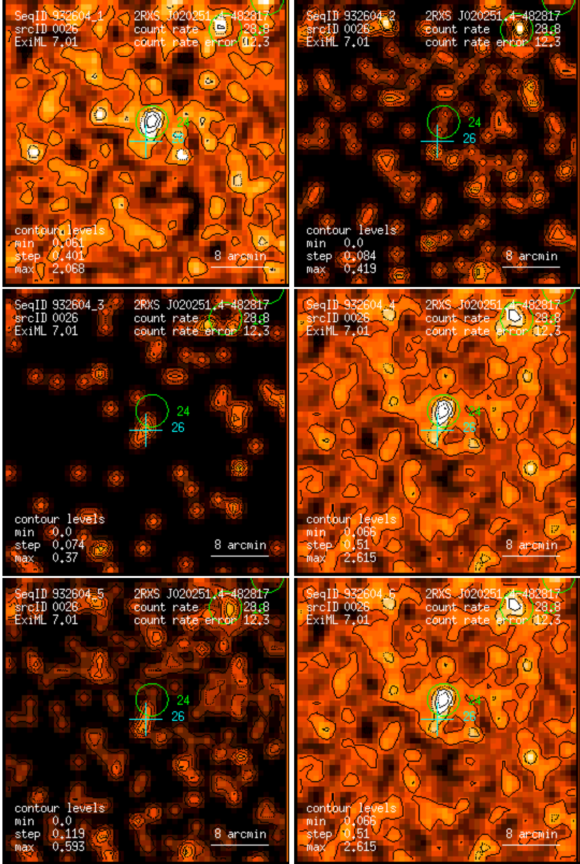
Figure 26: RASS 932604: detection 0026: band rate images, Gaussian filter: (1) PSPC channels 11 – 41, (2) 52 – 90, (3) 91 – 201, (4) 11 – 235, (5) 52 – 201, (6) 11 – 201. Broad band rates in counts/ks. Band rate contour levels in counts/ks/arcmin 2 .
