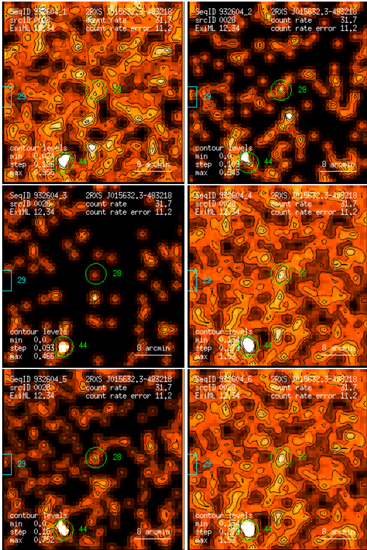
Figure 28: RASS 932604: detection 0028: band rate images, Gaussian filter: (1) PSPC channels 11 – 41, (2) 52 – 90, (3) 91 – 201, (4) 11 – 235, (5) 52 – 201, (6) 11 – 201. Broad band rates in counts/ks. Band rate contour levels in counts/ks/arcmin 2 .
