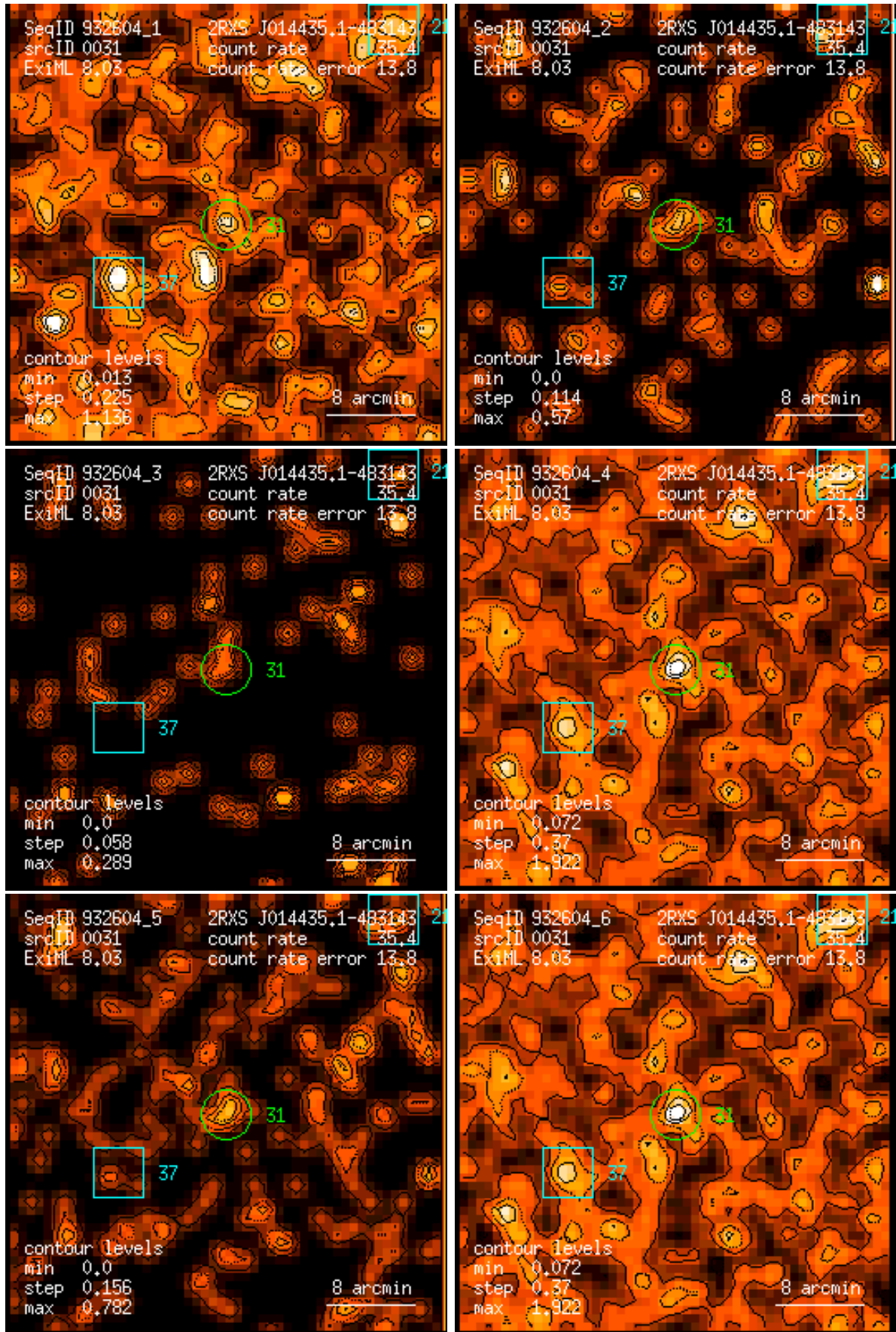
Figure 31: RASS 932604: detection 0031: band rate images, Gaussian filter: (1) PSPC channels 11 – 41, (2) 52 – 90, (3) 91 – 201, (4) 11 – 235, (5) 52 – 201, (6) 11 – 201. Broad band rates in counts/ks. Band rate contour levels in counts/ks/arcmin 2 .
