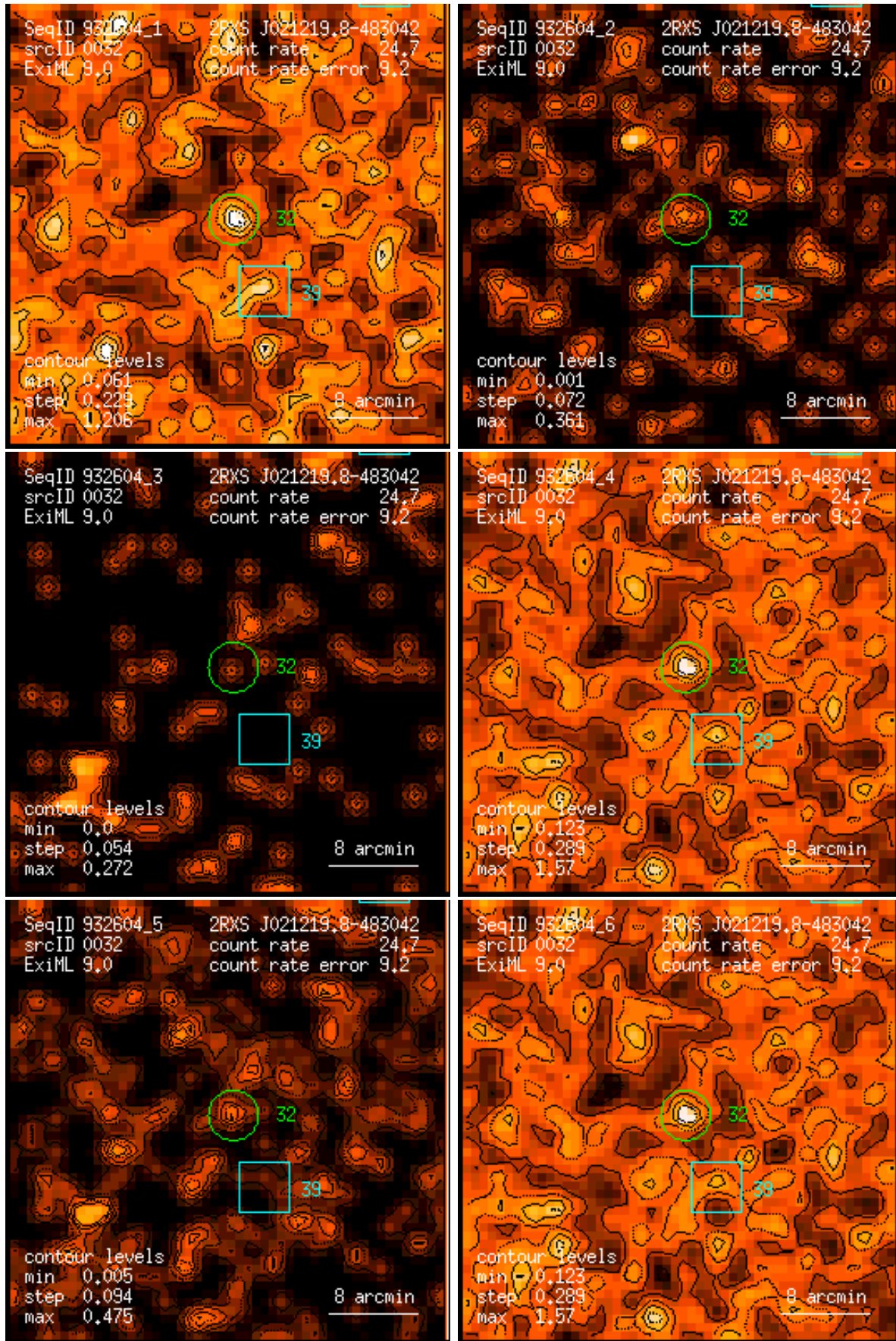
Figure 32: RASS 932604: detection 0032: band rate images, Gaussian filter: (1) PSPC channels 11 – 41, (2) 52 – 90, (3) 91 – 201, (4) 11 – 235, (5) 52 – 201, (6) 11 – 201. Broad band rates in counts/ks. Band rate contour levels in counts/ks/arcmin 2 .
