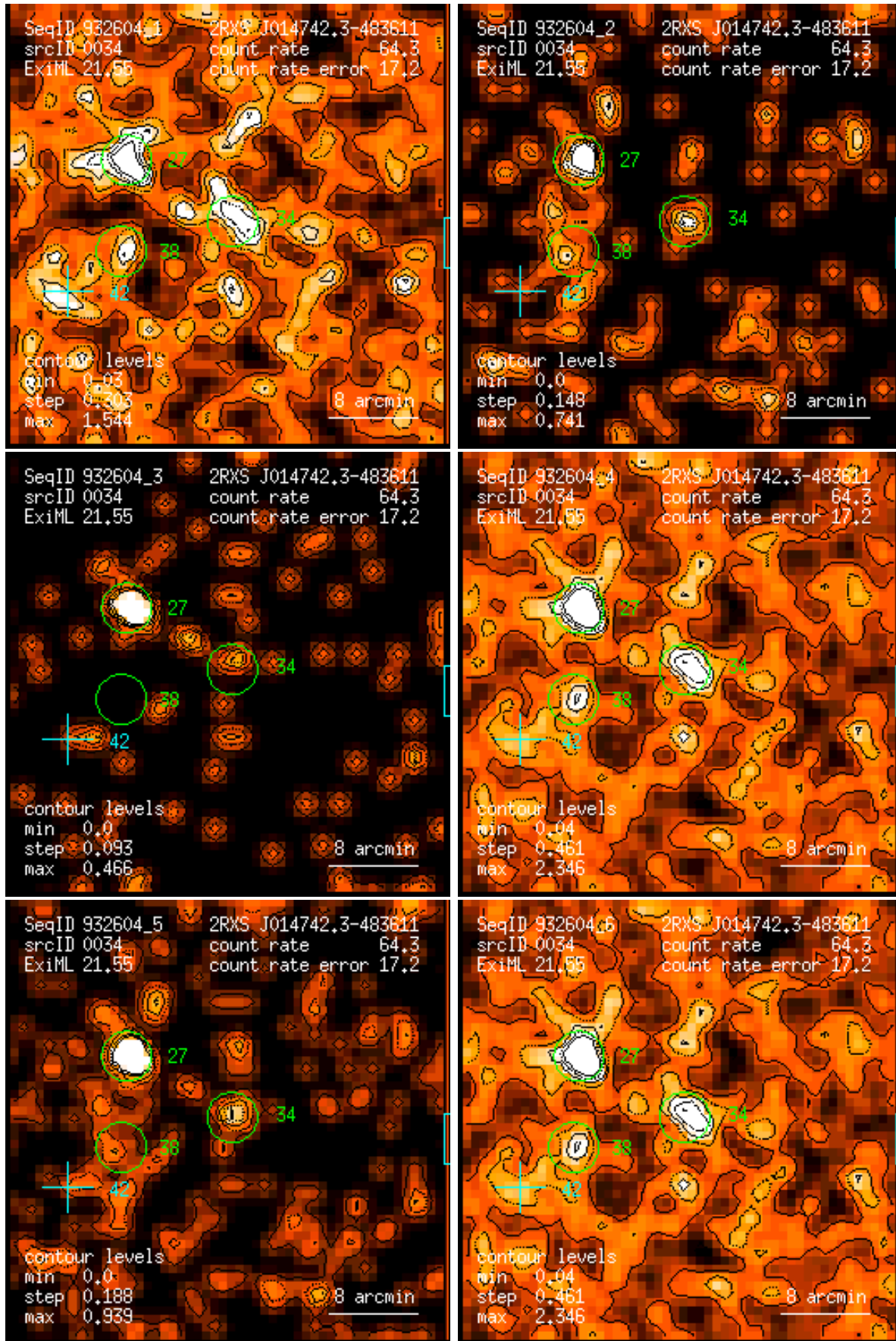
Figure 34: RASS 932604: detection 0034: band rate images, Gaussian filter: (1) PSPC channels 11 – 41, (2) 52 – 90, (3) 91 – 201, (4) 11 – 235, (5) 52 – 201, (6) 11 – 201. Broad band rates in counts/ks. Band rate contour levels in counts/ks/arcmin 2 .
