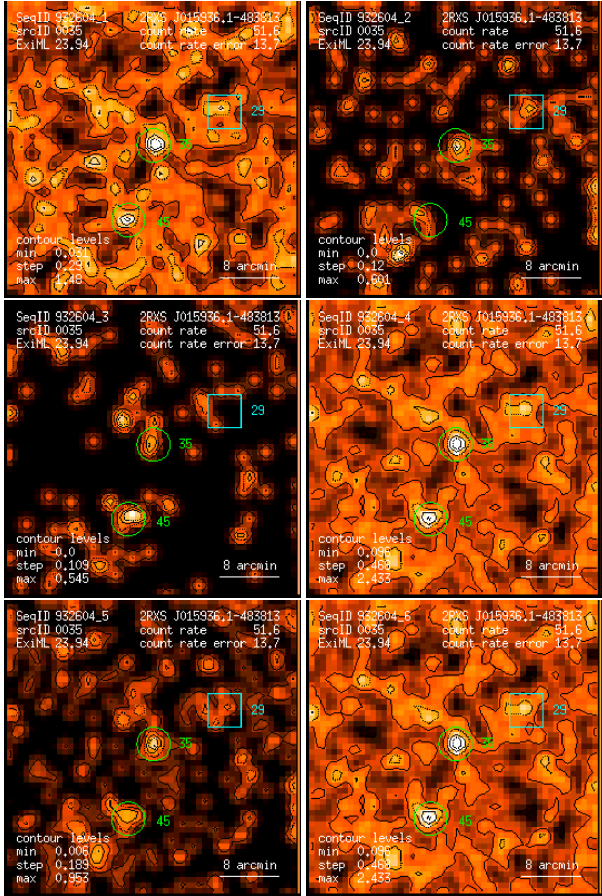
Figure 35: RASS 932604: detection 0035: band rate images, Gaussian filter: (1) PSPC channels 11 – 41, (2) 52 – 90, (3) 91 – 201, (4) 11 – 235, (5) 52 – 201, (6) 11 – 201. Broad band rates in counts/ks. Band rate contour levels in counts/ks/arcmin 2 .
