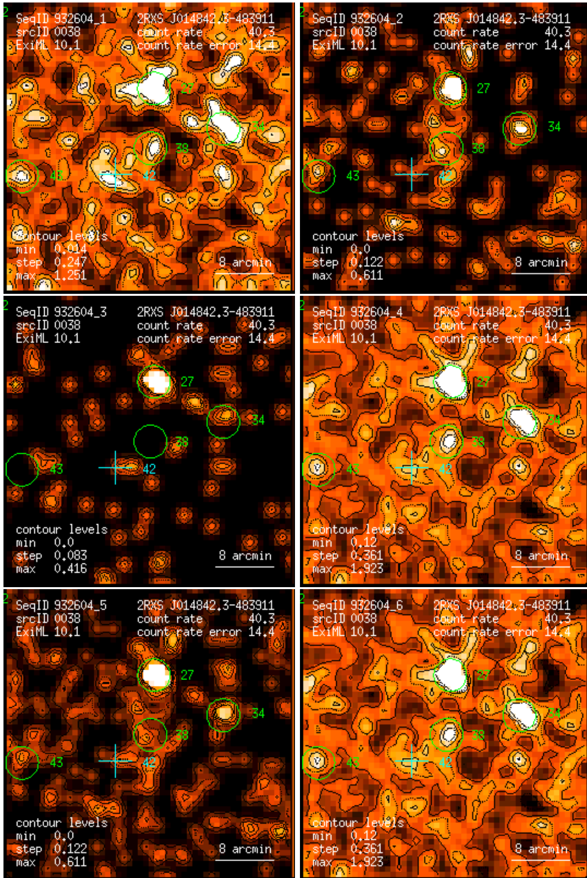
Figure 38: RASS 932604: detection 0038: band rate images, Gaussian filter: (1) PSPC channels 11 – 41, (2) 52 – 90, (3) 91 – 201, (4) 11 – 235, (5) 52 – 201, (6) 11 – 201. Broad band rates in counts/ks. Band rate contour levels in counts/ks/arcmin 2 .
