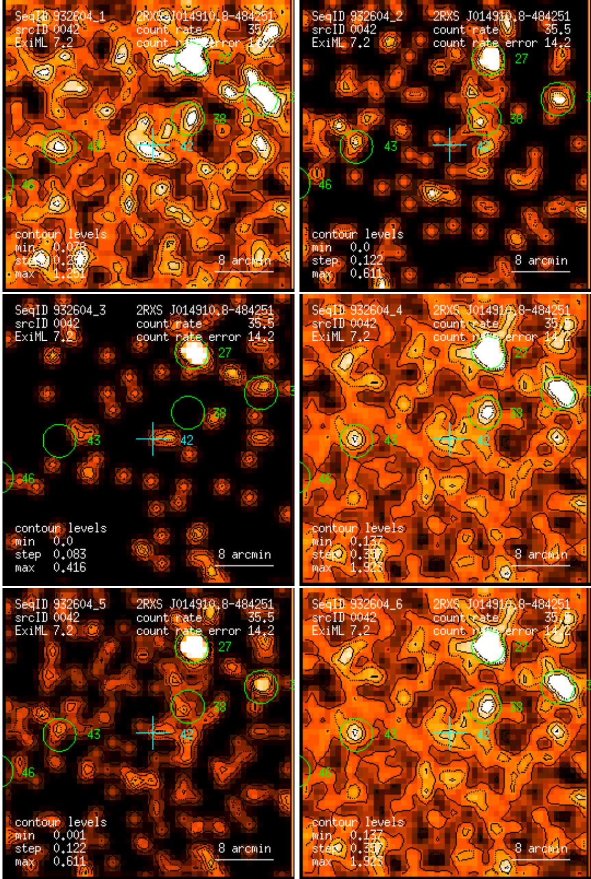
Figure 42: RASS 932604: detection 0042: band rate images, Gaussian filter: (1) PSPC channels 11 – 41, (2) 52 – 90, (3) 91 – 201, (4) 11 – 235, (5) 52 – 201, (6) 11 – 201. Broad band rates in counts/ks. Band rate contour levels in counts/ks/arcmin 2 .
