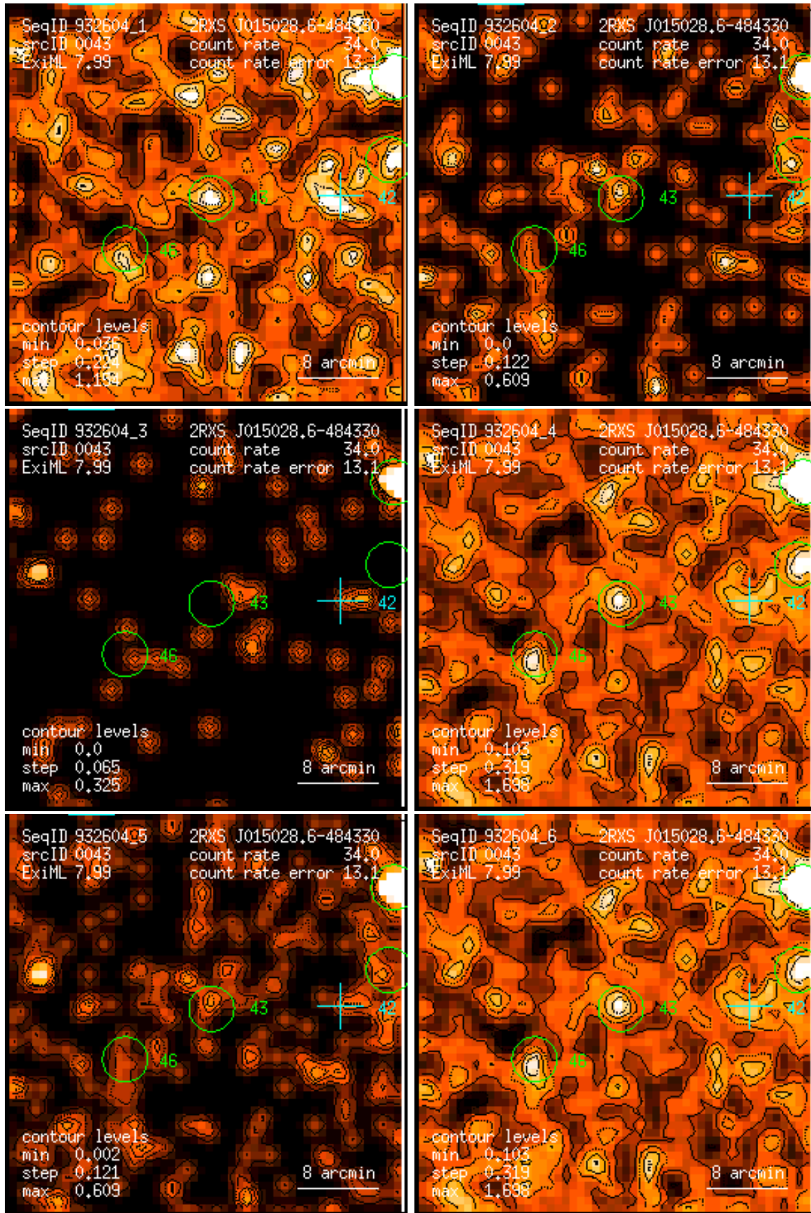
Figure 43: RASS 932604: detection 0043: band rate images, Gaussian filter: (1) PSPC channels 11 – 41, (2) 52 – 90, (3) 91 – 201, (4) 11 – 235, (5) 52 – 201, (6) 11 – 201. Broad band rates in counts/ks. Band rate contour levels in counts/ks/arcmin 2 .
