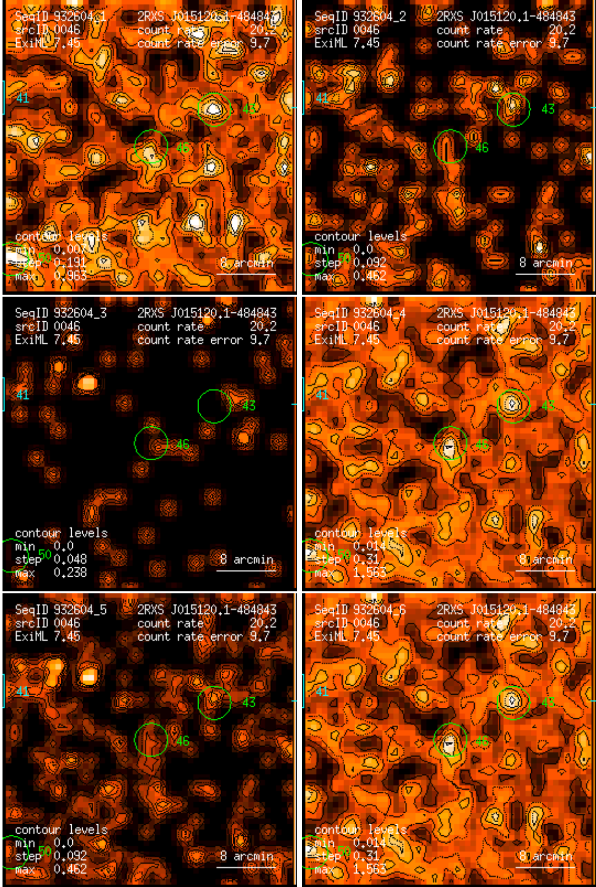
Figure 46: RASS 932604: detection 0046: band rate images, Gaussian filter: (1) PSPC channels 11 – 41, (2) 52 – 90, (3) 91 – 201, (4) 11 – 235, (5) 52 – 201, (6) 11 – 201. Broad band rates in counts/ks. Band rate contour levels in counts/ks/arcmin 2 .
