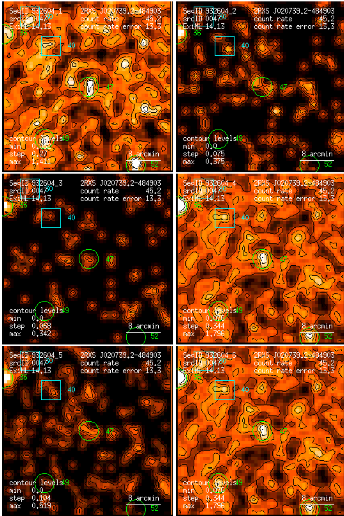
Figure 47: RASS 932604: detection 0047: band rate images, Gaussian filter: (1) PSPC channels 11 – 41, (2) 52 – 90, (3) 91 – 201, (4) 11 – 235, (5) 52 – 201, (6) 11 – 201. Broad band rates in counts/ks. Band rate contour levels in counts/ks/arcmin 2 .
