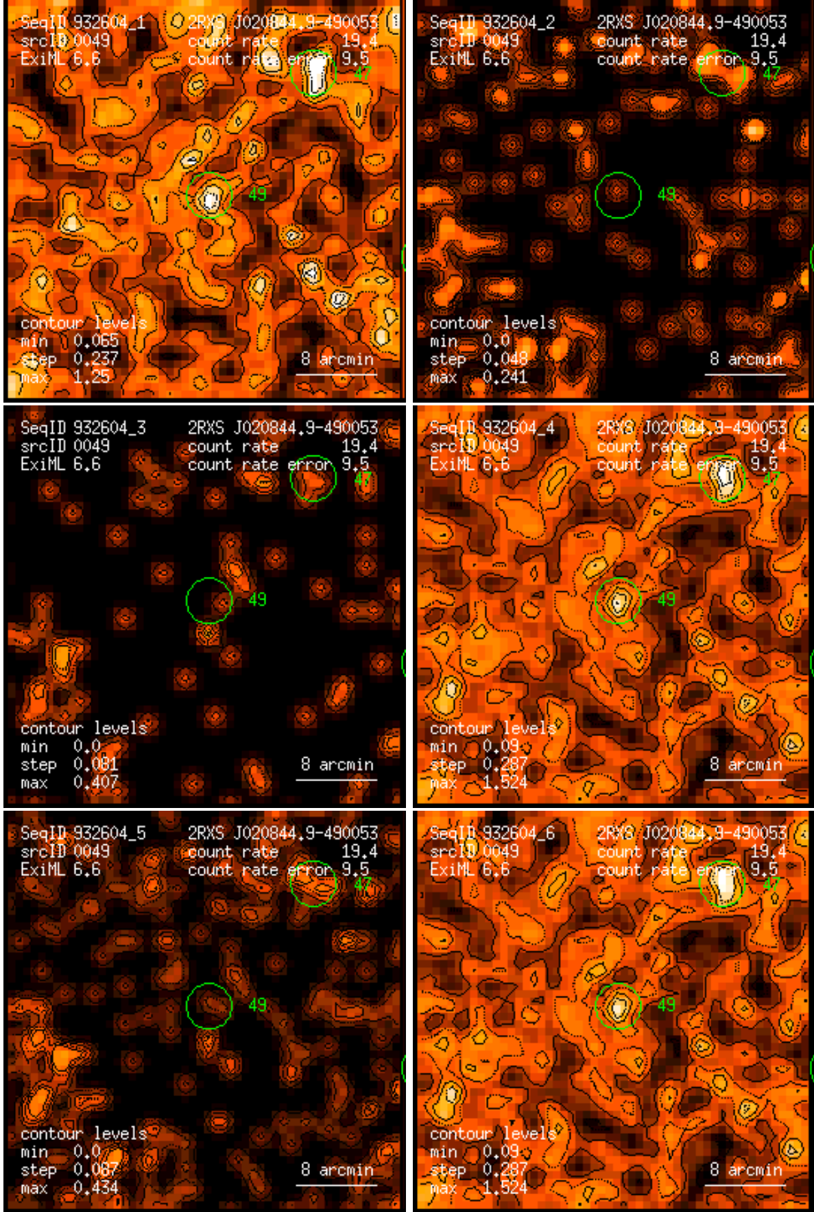
Figure 49: RASS 932604: detection 0049: band rate images, Gaussian filter: (1) PSPC channels 11 – 41, (2) 52 – 90, (3) 91 – 201, (4) 11 – 235, (5) 52 – 201, (6) 11 – 201. Broad band rates in counts/ks. Band rate contour levels in counts/ks/arcmin 2 .
