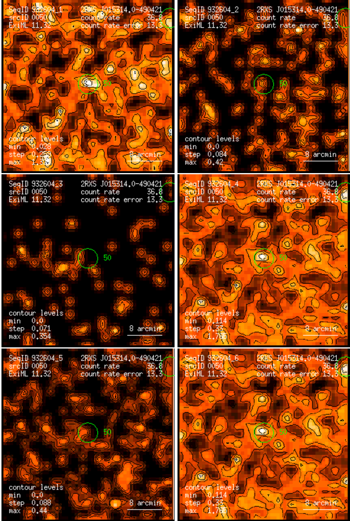
Figure 50: RASS 932604: detection 0050: band rate images, Gaussian filter: (1) PSPC channels 11 – 41, (2) 52 – 90, (3) 91 – 201, (4) 11 – 235, (5) 52 – 201, (6) 11 – 201. Broad band rates in counts/ks. Band rate contour levels in counts/ks/arcmin 2 .
