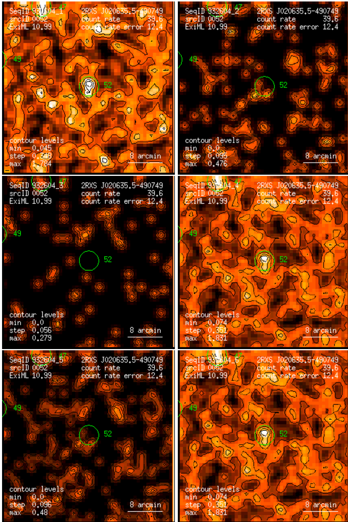
Figure 52: RASS 932604: detection 0052: band rate images, Gaussian filter: (1) PSPC channels 11 – 41, (2) 52 – 90, (3) 91 – 201, (4) 11 – 235, (5) 52 – 201, (6) 11 – 201. Broad band rates in counts/ks. Band rate contour levels in counts/ks/arcmin 2 .
