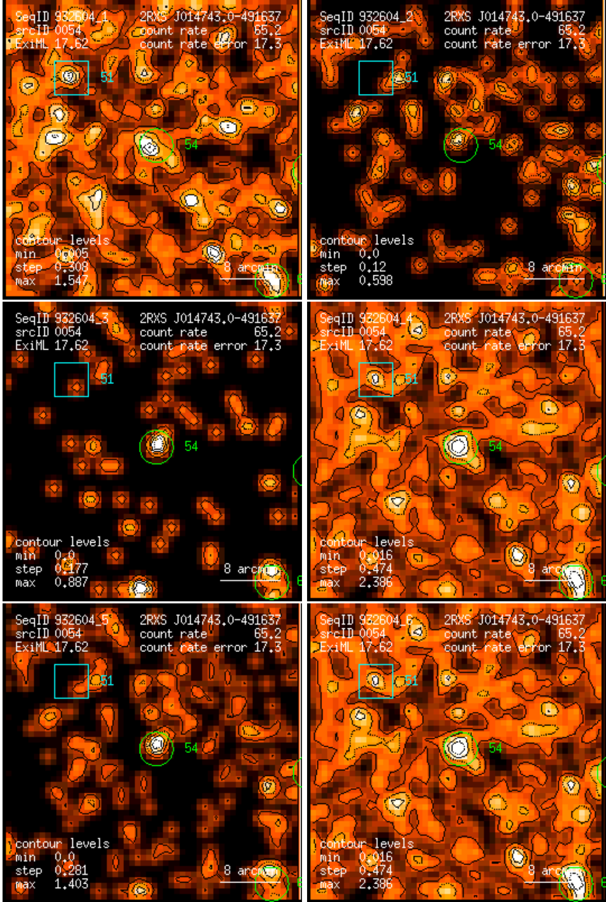
Figure 54: RASS 932604: detection 0054: band rate images, Gaussian filter: (1) PSPC channels 11 – 41, (2) 52 – 90, (3) 91 – 201, (4) 11 – 235, (5) 52 – 201, (6) 11 – 201. Broad band rates in counts/ks. Band rate contour levels in counts/ks/arcmin 2 .
