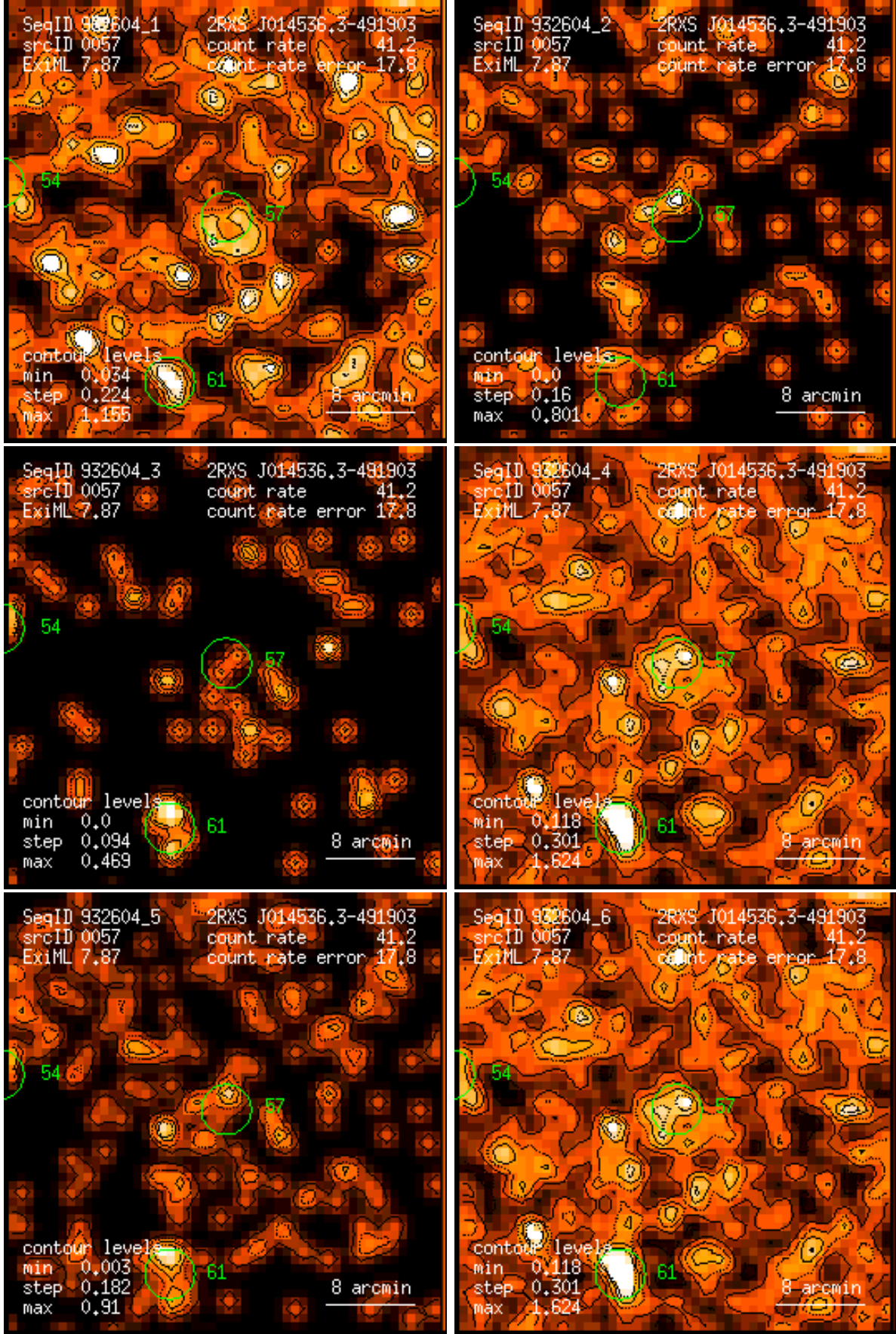
Figure 57: RASS 932604: detection 0057: band rate images, Gaussian filter: (1) PSPC channels 11 – 41, (2) 52 – 90, (3) 91 – 201, (4) 11 – 235, (5) 52 – 201, (6) 11 – 201. Broad band rates in counts/ks. Band rate contour levels in counts/ks/arcmin 2 .
