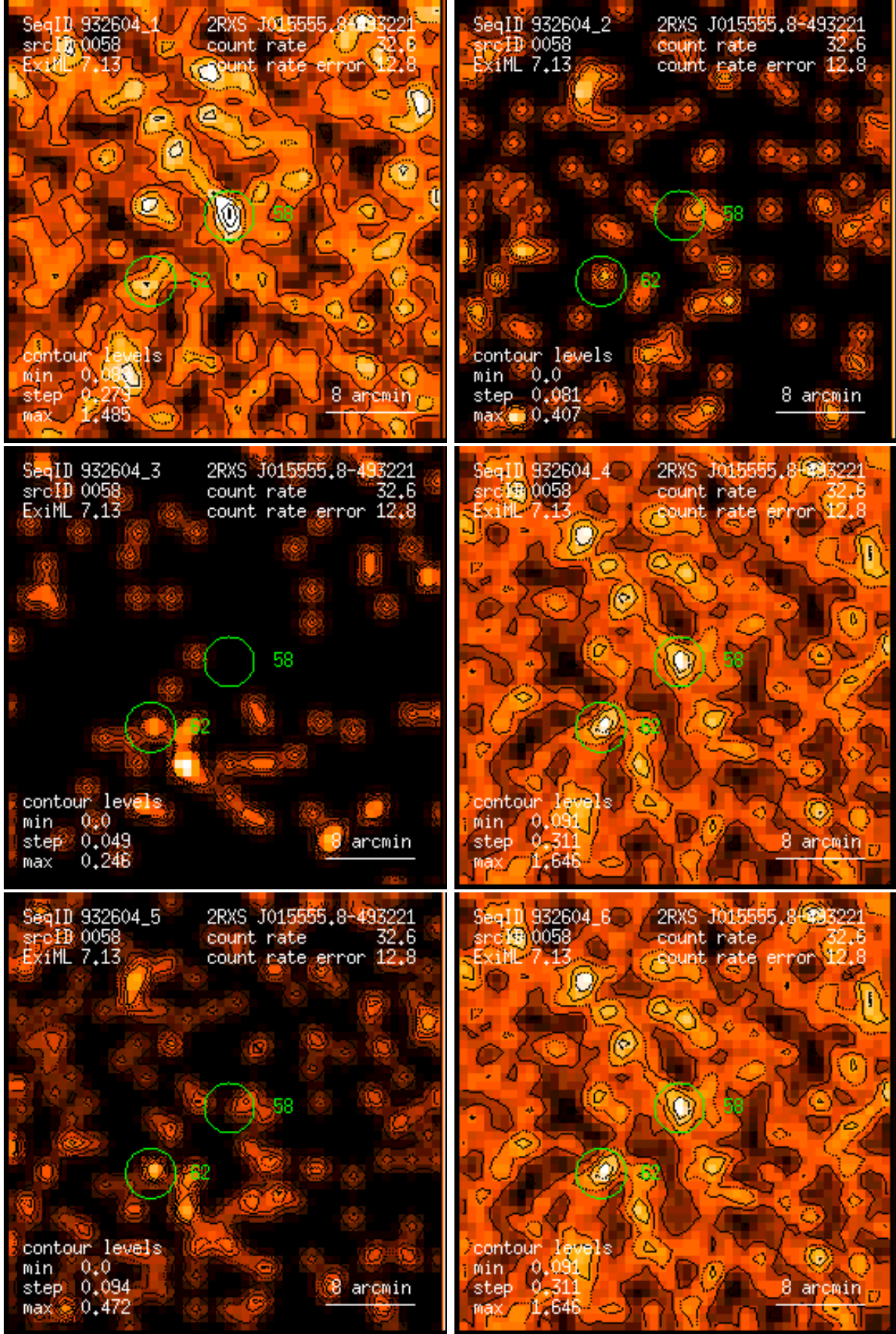
Figure 58: RASS 932604: detection 0058: band rate images, Gaussian filter: (1) PSPC channels 11 – 41, (2) 52 – 90, (3) 91 – 201, (4) 11 – 235, (5) 52 – 201, (6) 11 – 201. Broad band rates in counts/ks. Band rate contour levels in counts/ks/arcmin 2 .
