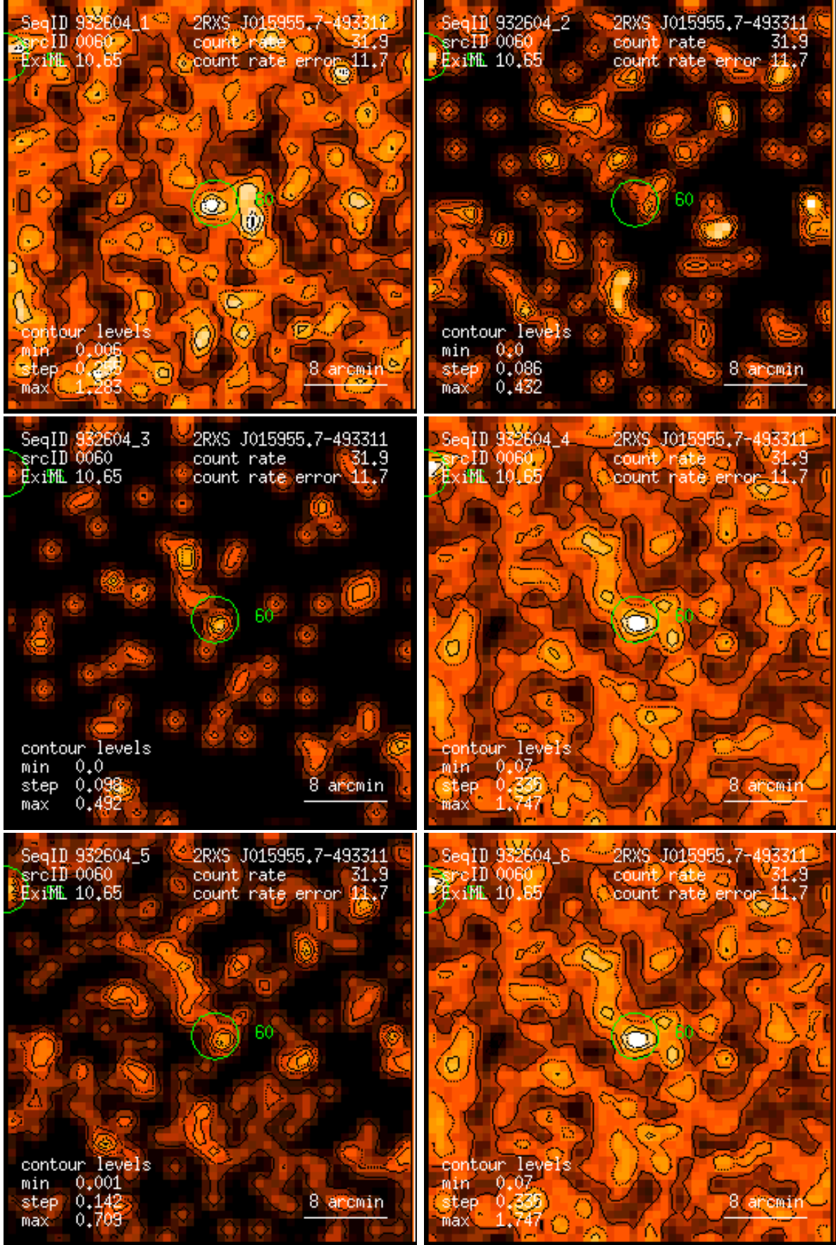
Figure 60: RASS 932604: detection 0060: band rate images, Gaussian filter: (1) PSPC channels 11 – 41, (2) 52 – 90, (3) 91 – 201, (4) 11 – 235, (5) 52 – 201, (6) 11 – 201. Broad band rates in counts/ks. Band rate contour levels in counts/ks/arcmin 2 .
