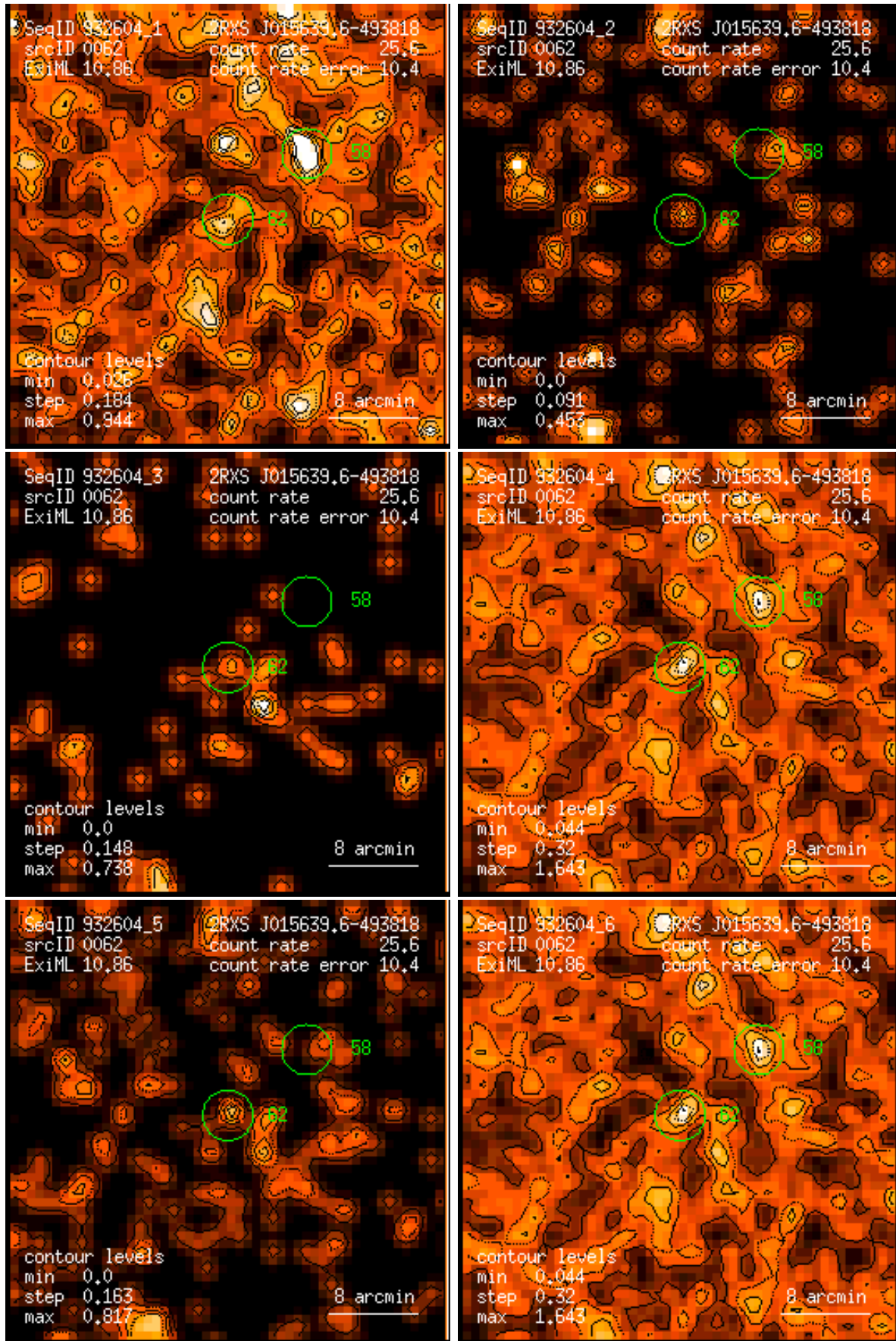
Figure 62: RASS 932604: detection 0062: band rate images, Gaussian filter: (1) PSPC channels 11 – 41, (2) 52 – 90, (3) 91 – 201, (4) 11 – 235, (5) 52 – 201, (6) 11 – 201. Broad band rates in counts/ks. Band rate contour levels in counts/ks/arcmin 2 .
