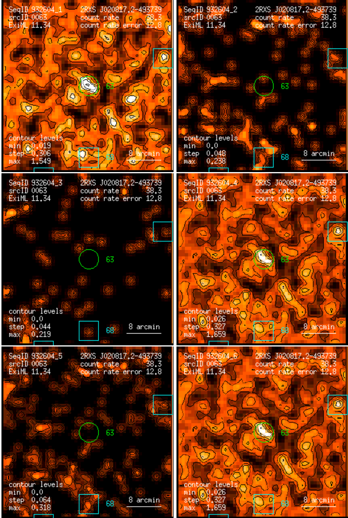
Figure 63: RASS 932604: detection 0063: band rate images, Gaussian filter: (1) PSPC channels 11 – 41, (2) 52 – 90, (3) 91 – 201, (4) 11 – 235, (5) 52 – 201, (6) 11 – 201. Broad band rates in counts/ks. Band rate contour levels in counts/ks/arcmin 2 .
