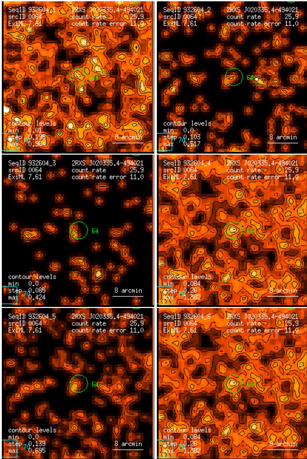
Figure 64: RASS 932604: detection 0064: band rate images, Gaussian filter: (1) PSPC channels 11 – 41, (2) 52 – 90, (3) 91 – 201, (4) 11 – 235, (5) 52 – 201, (6) 11 – 201. Broad band rates in counts/ks. Band rate contour levels in counts/ks/arcmin 2 .
