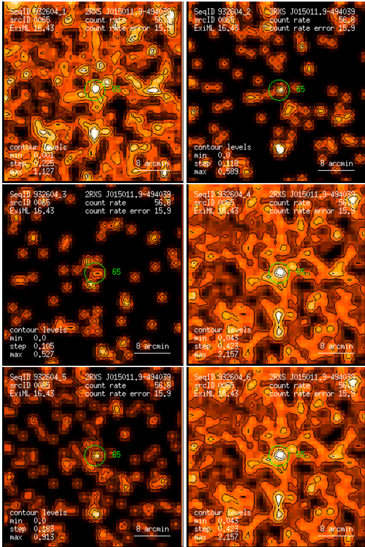
Figure 65: RASS 932604: detection 0065: band rate images, Gaussian filter: (1) PSPC channels 11 – 41, (2) 52 – 90, (3) 91 – 201, (4) 11 – 235, (5) 52 – 201, (6) 11 – 201. Broad band rates in counts/ks. Band rate contour levels in counts/ks/arcmin 2 .
