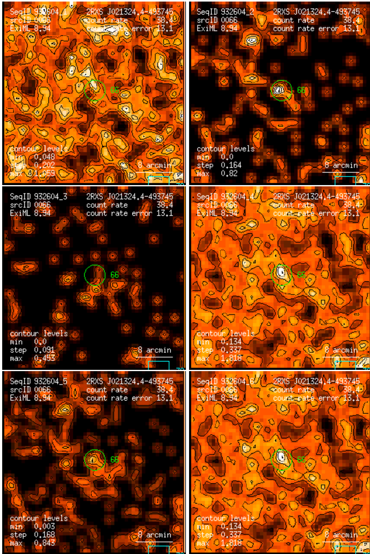
Figure 66: RASS 932604: detection 0066: band rate images, Gaussian filter: (1) PSPC channels 11 – 41, (2) 52 – 90, (3) 91 – 201, (4) 11 – 235, (5) 52 – 201, (6) 11 – 201. Broad band rates in counts/ks. Band rate contour levels in counts/ks/arcmin 2 .
