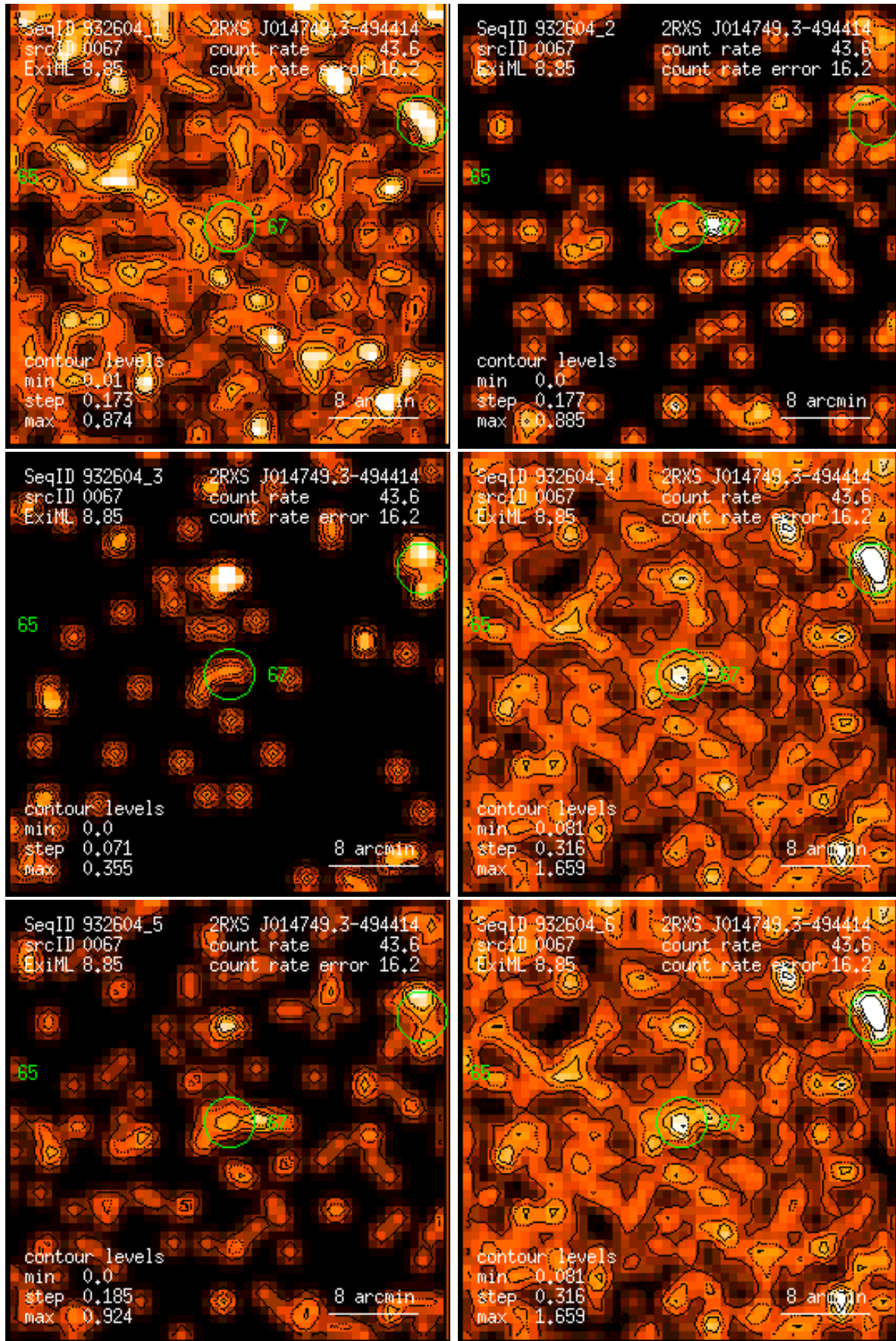
Figure 67: RASS 932604: detection 0067: band rate images, Gaussian filter: (1) PSPC channels 11 – 41, (2) 52 – 90, (3) 91 – 201, (4) 11 – 235, (5) 52 – 201, (6) 11 – 201. Broad band rates in counts/ks. Band rate contour levels in counts/ks/arcmin 2 .
