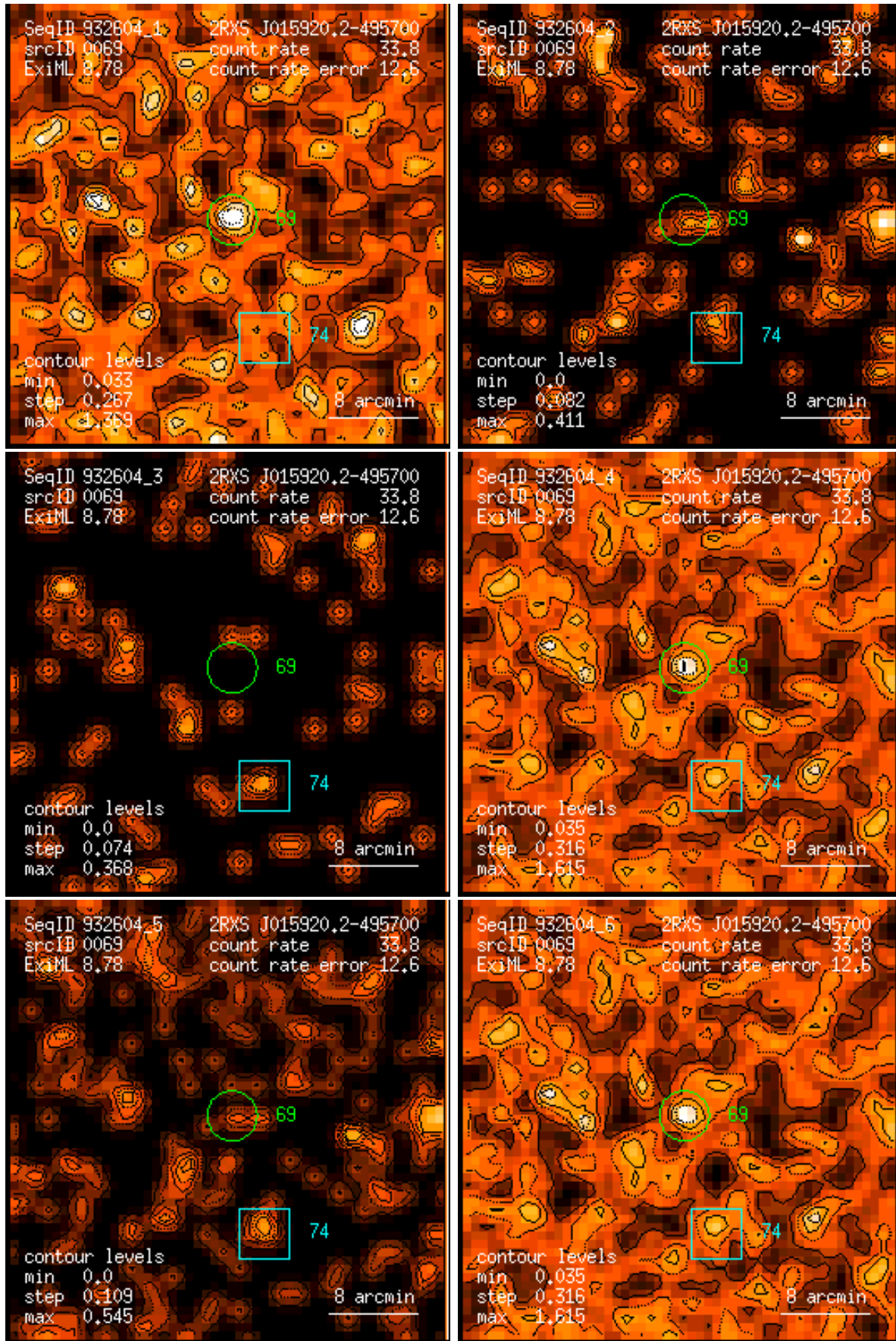
Figure 69: RASS 932604: detection 0069: band rate images, Gaussian filter: (1) PSPC channels 11 – 41, (2) 52 – 90, (3) 91 – 201, (4) 11 – 235, (5) 52 – 201, (6) 11 – 201. Broad band rates in counts/ks. Band rate contour levels in counts/ks/arcmin 2 .
