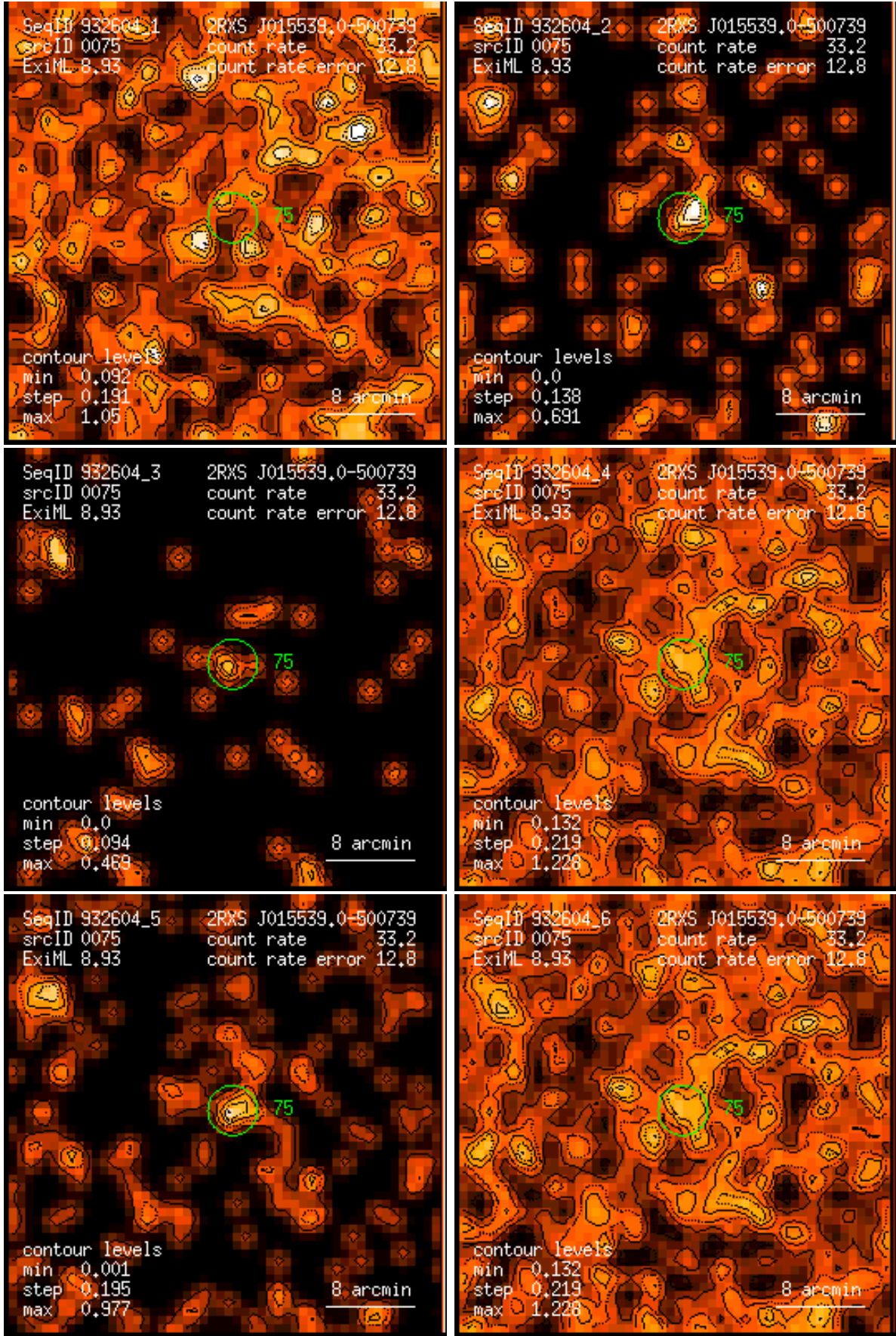
Figure 75: RASS 932604: detection 0075: band rate images, Gaussian filter: (1) PSPC channels 11 – 41, (2) 52 – 90, (3) 91 – 201, (4) 11 – 235, (5) 52 – 201, (6) 11 – 201. Broad band rates in counts/ks. Band rate contour levels in counts/ks/arcmin 2 .
