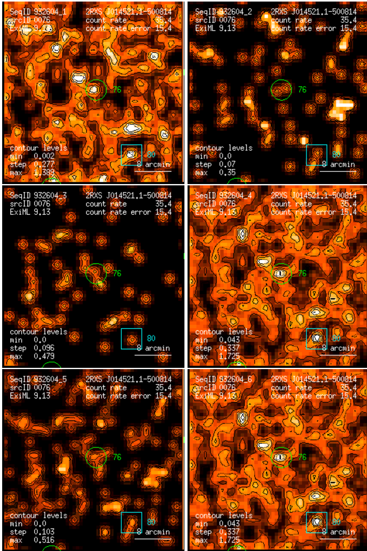
Figure 76: RASS 932604: detection 0076: band rate images, Gaussian filter: (1) PSPC channels 11 – 41, (2) 52 – 90, (3) 91 – 201, (4) 11 – 235, (5) 52 – 201, (6) 11 – 201. Broad band rates in counts/ks. Band rate contour levels in counts/ks/arcmin 2 .
