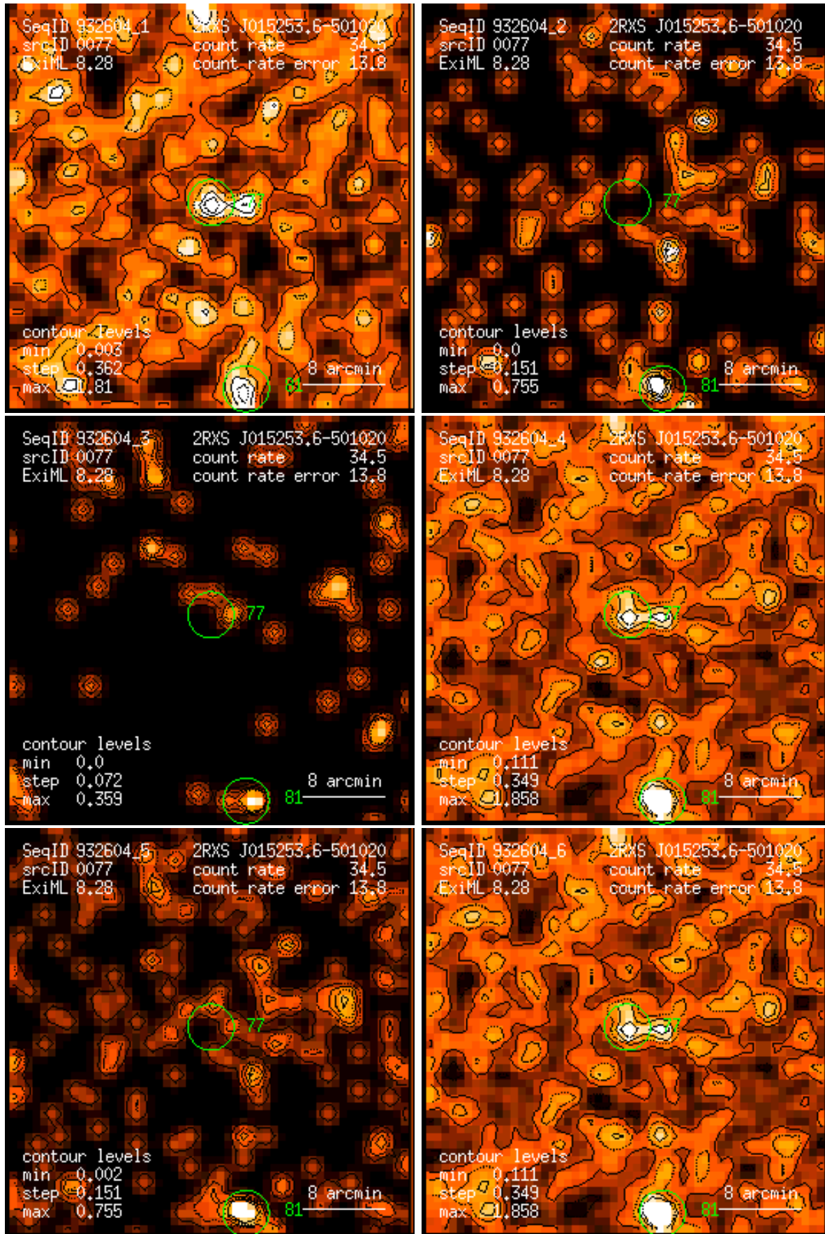
Figure 77: RASS 932604: detection 0077: band rate images, Gaussian filter: (1) PSPC channels 11 – 41, (2) 52 – 90, (3) 91 – 201, (4) 11 – 235, (5) 52 – 201, (6) 11 – 201. Broad band rates in counts/ks. Band rate contour levels in counts/ks/arcmin 2 .
