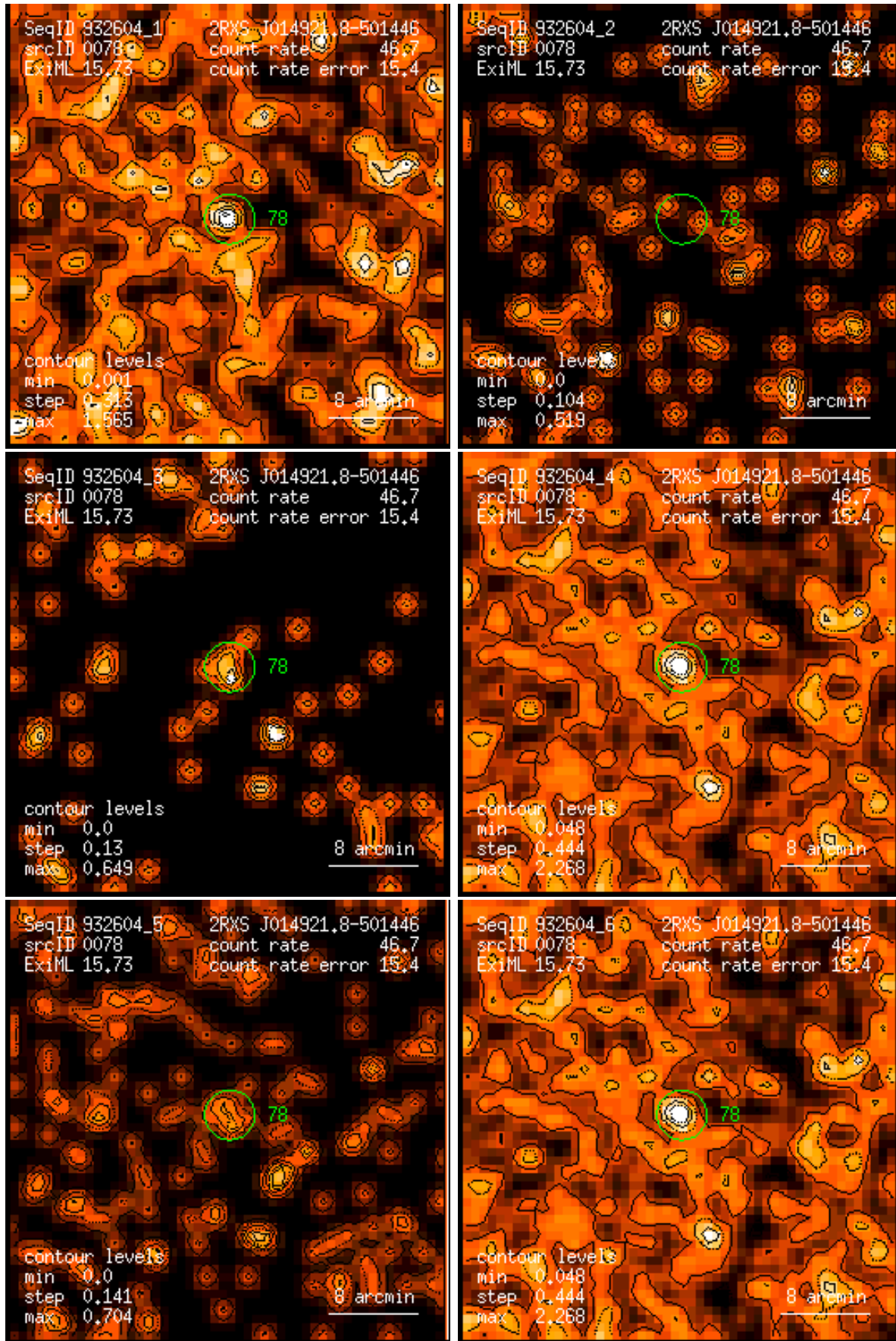
Figure 78: RASS 932604: detection 0078: band rate images, Gaussian filter: (1) PSPC channels 11 – 41, (2) 52 – 90, (3) 91 – 201, (4) 11 – 235, (5) 52 – 201, (6) 11 – 201. Broad band rates in counts/ks. Band rate contour levels in counts/ks/arcmin 2 .
