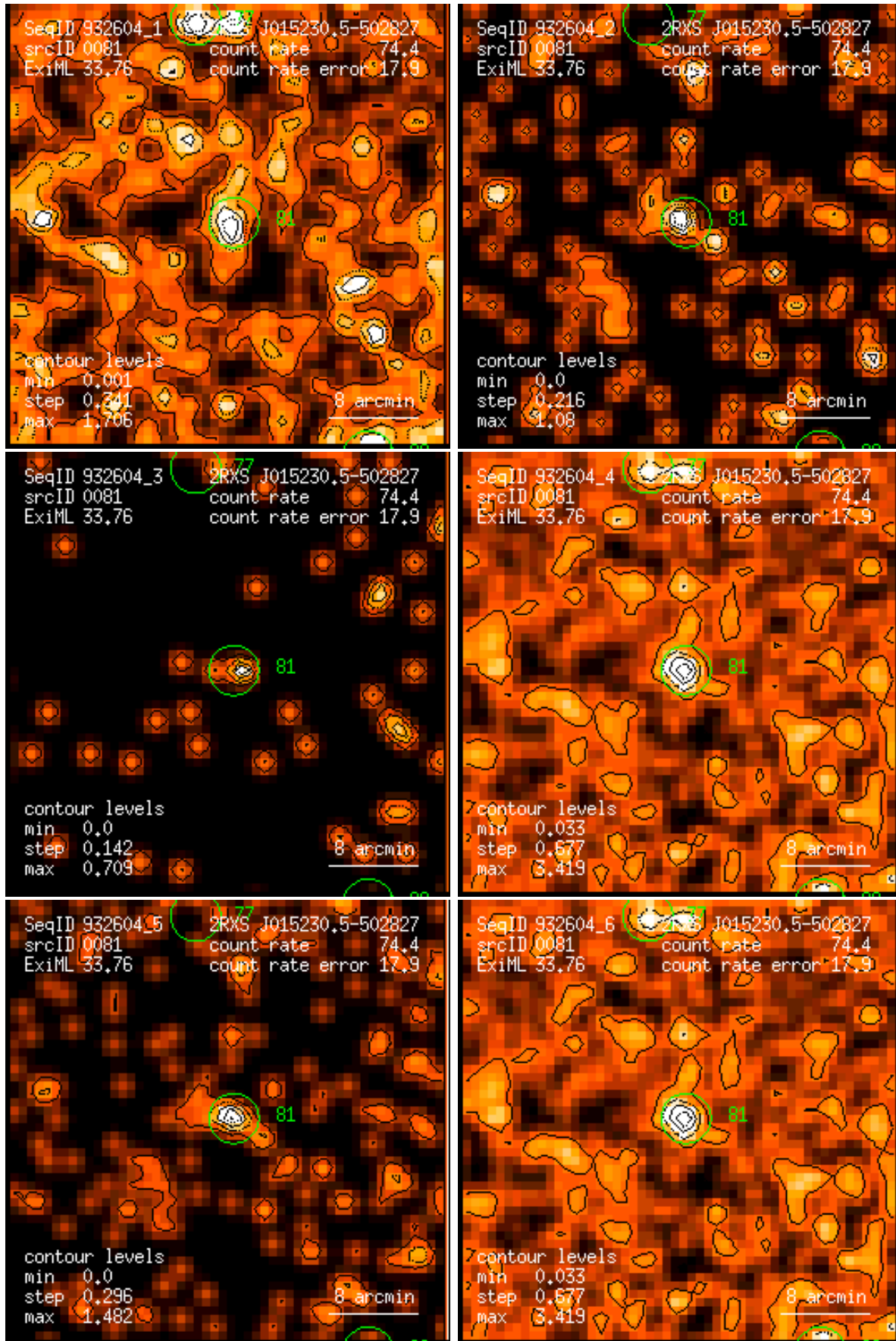
Figure 81: RASS 932604: detection 0081: band rate images, Gaussian filter: (1) PSPC channels 11 – 41, (2) 52 – 90, (3) 91 – 201, (4) 11 – 235, (5) 52 – 201, (6) 11 – 201. Broad band rates in counts/ks. Band rate contour levels in counts/ks/arcmin 2 .
