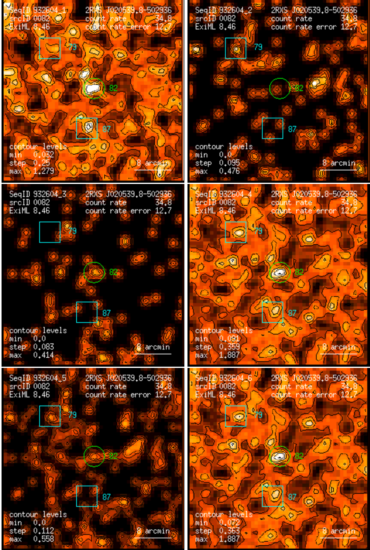
Figure 82: RASS 932604: detection 0082: band rate images, Gaussian filter: (1) PSPC channels 11 – 41, (2) 52 – 90, (3) 91 – 201, (4) 11 – 235, (5) 52 – 201, (6) 11 – 201. Broad band rates in counts/ks. Band rate contour levels in counts/ks/arcmin 2 .
