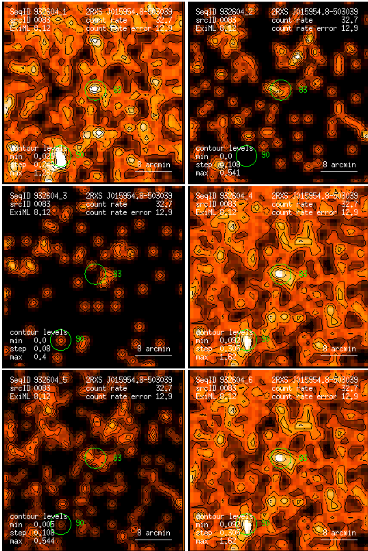
Figure 83: RASS 932604: detection 0083: band rate images, Gaussian filter: (1) PSPC channels 11 – 41, (2) 52 – 90, (3) 91 – 201, (4) 11 – 235, (5) 52 – 201, (6) 11 – 201. Broad band rates in counts/ks. Band rate contour levels in counts/ks/arcmin 2 .
