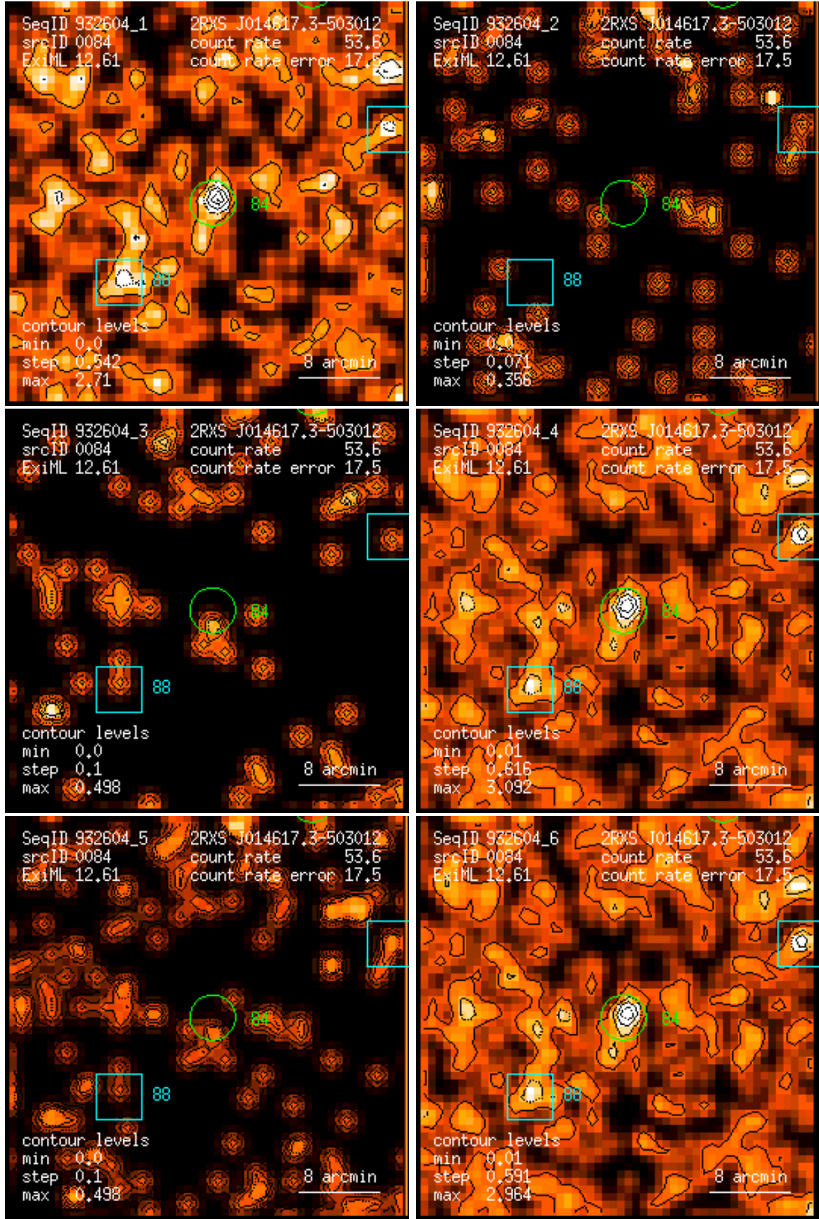
Figure 84: RASS 932604: detection 0084: band rate images, Gaussian filter: (1) PSPC channels 11 – 41, (2) 52 – 90, (3) 91 – 201, (4) 11 – 235, (5) 52 – 201, (6) 11 – 201. Broad band rates in counts/ks. Band rate contour levels in counts/ks/arcmin 2 .
